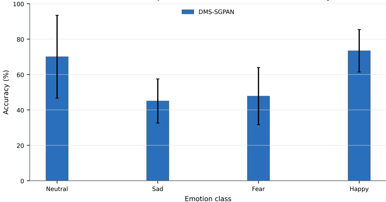
SEED-IV: class-wise performance on held-out TVT test subjects
