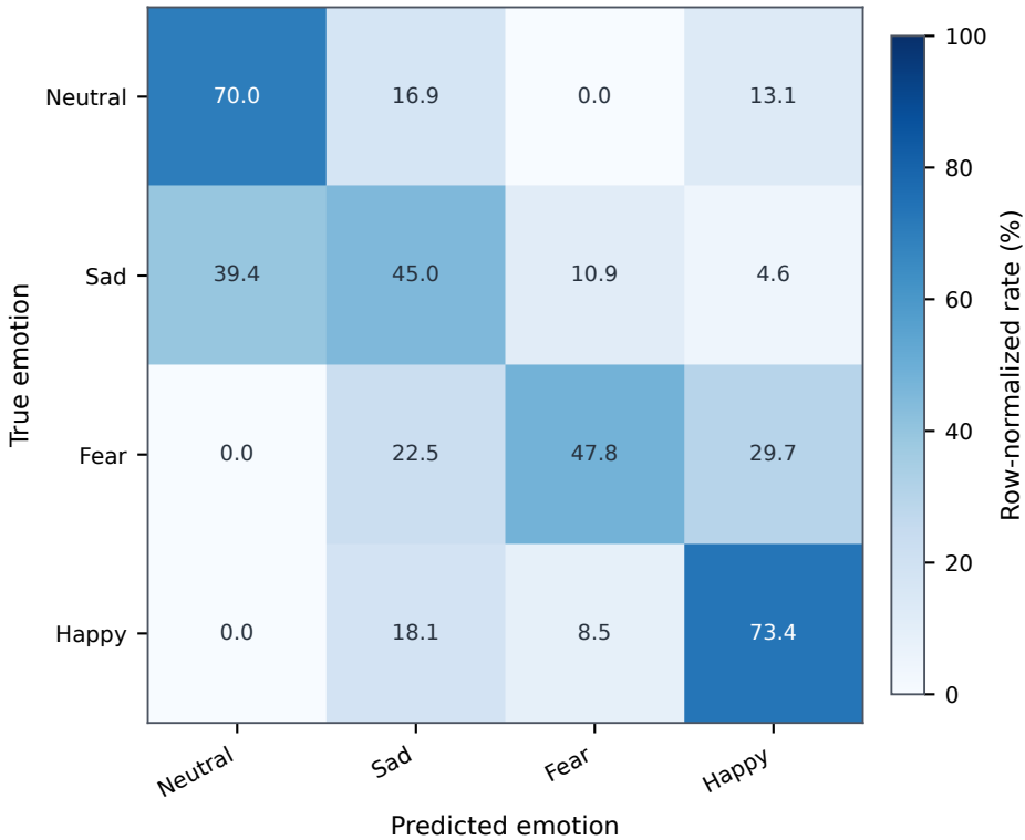
SEED-IV: DMS-SGPAN confusion matrix
