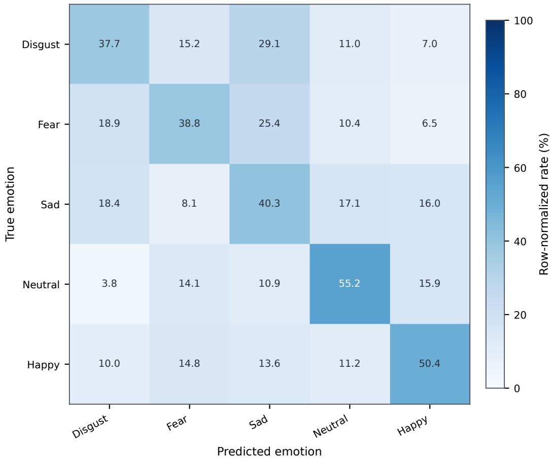
SEED-V: DMS-SGPAN confusion matrix
