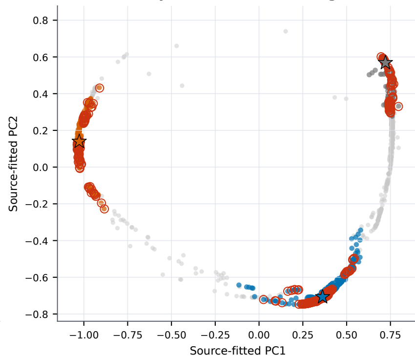
(b) Reliability filter ( \tau=0.95 ; coverage=81.2%)
