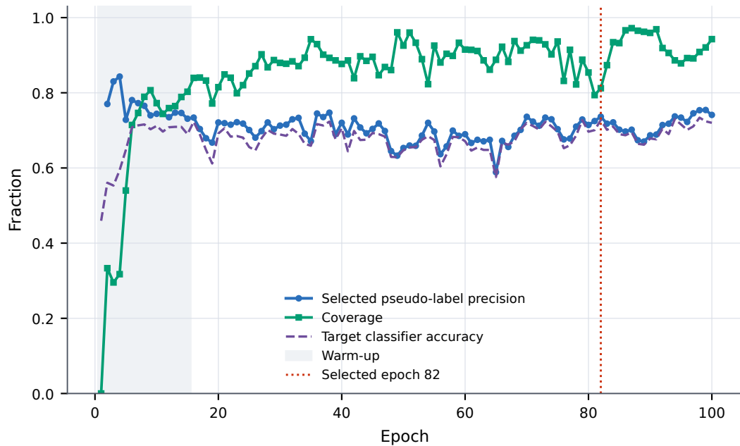
(a) Training trajectory at \tau=0.95
