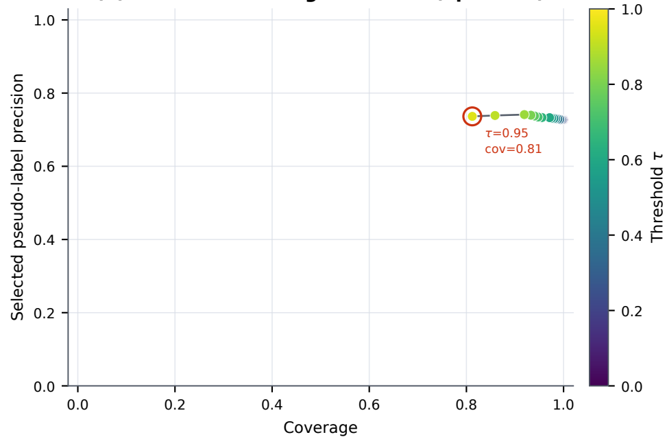
(b) Precision-coverage trade-off (epoch 82)
