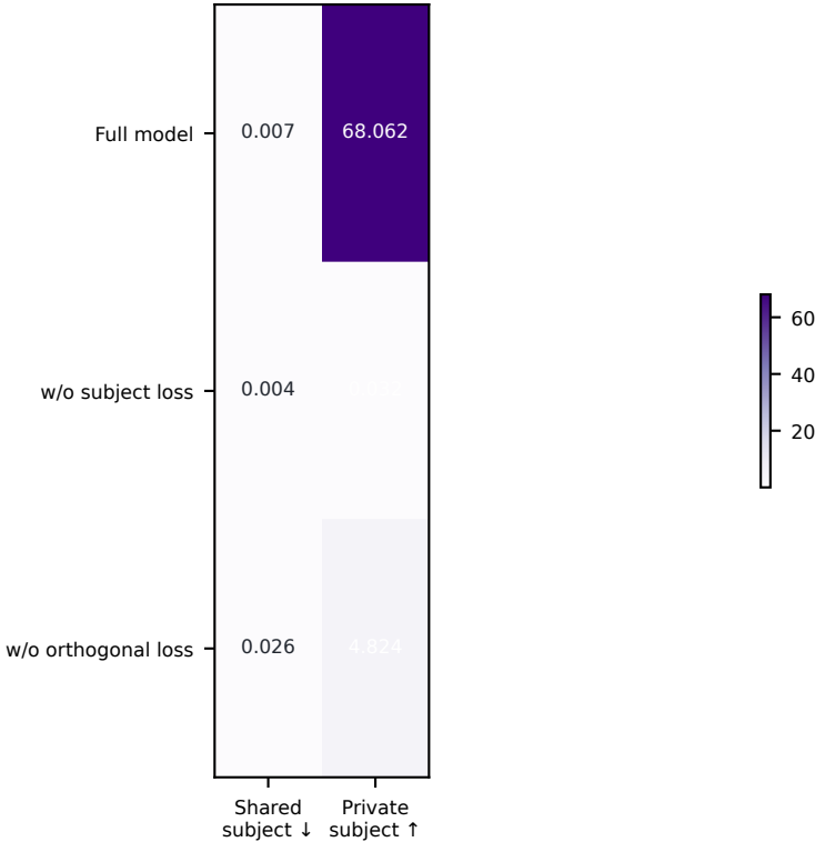
(c) Shared/private factorization
