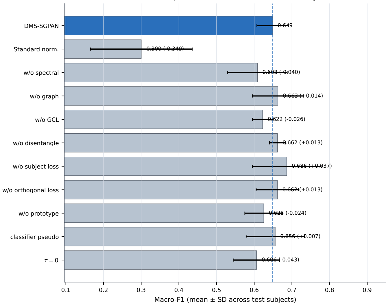
Ablation comparison on the held-out test subjects
