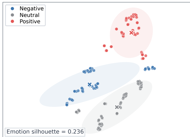
(a) SEED
