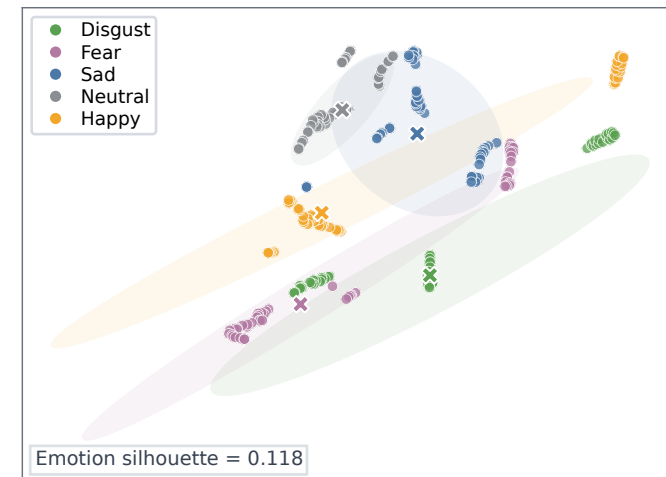
(c) SEED-V
