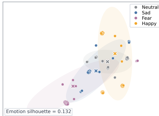
(b) SEED-IV
