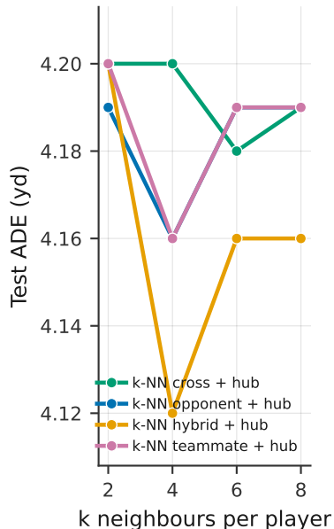
(b) k sweep, hub topologies
