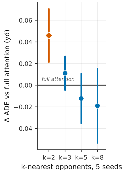
(c) No mask is significantly better
