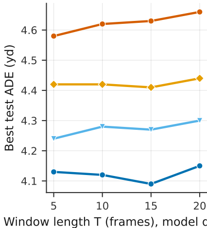
(b) History length
