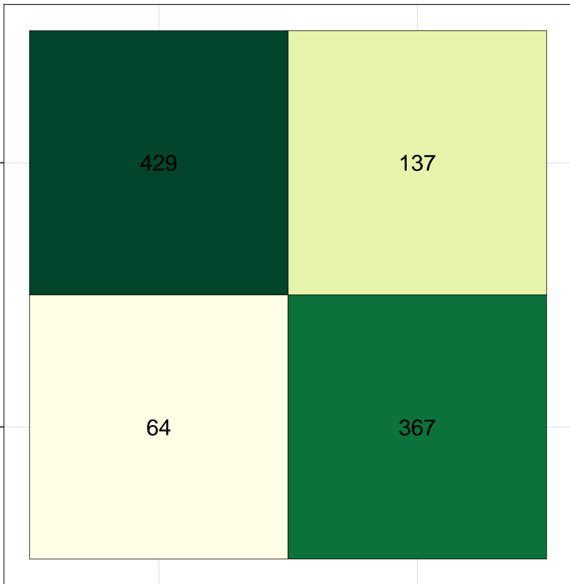
Confusion Matrix
