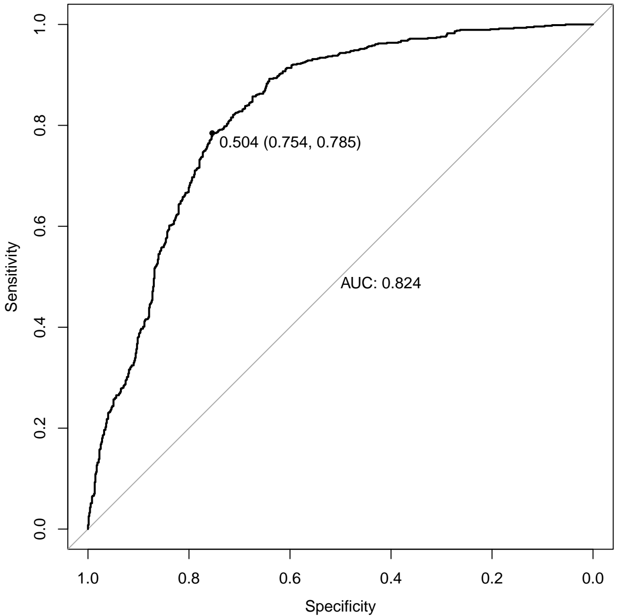
ROC Plot Ridge
