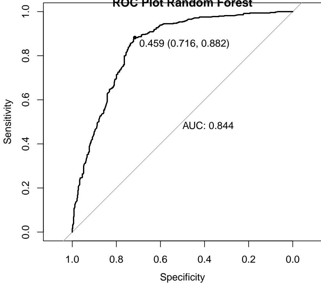
ROC Plot Random Forest
