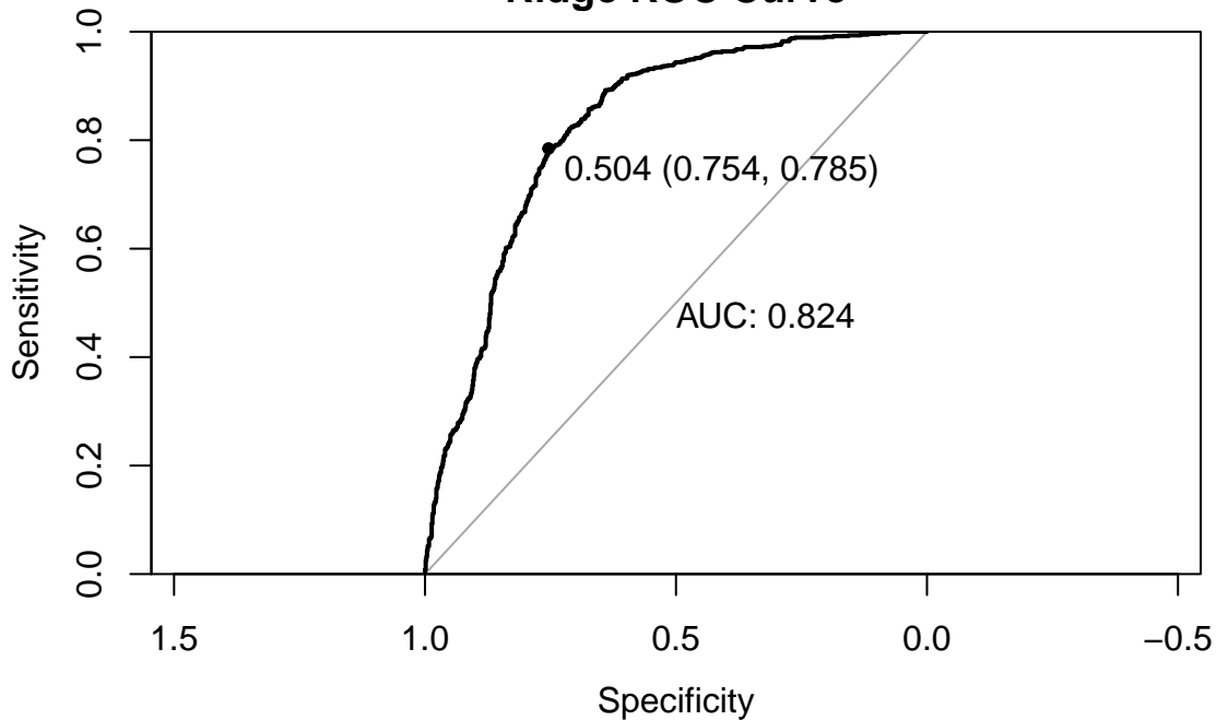
Ridge ROC Curve
