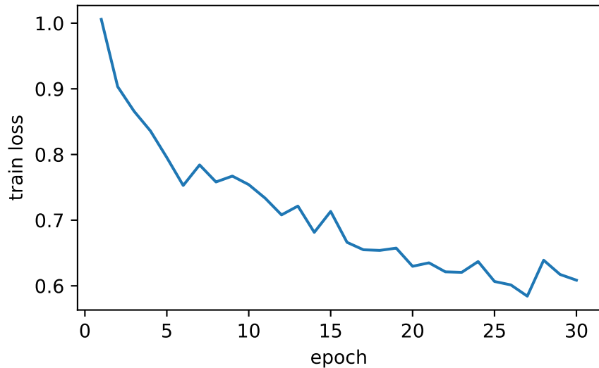
Training loss
