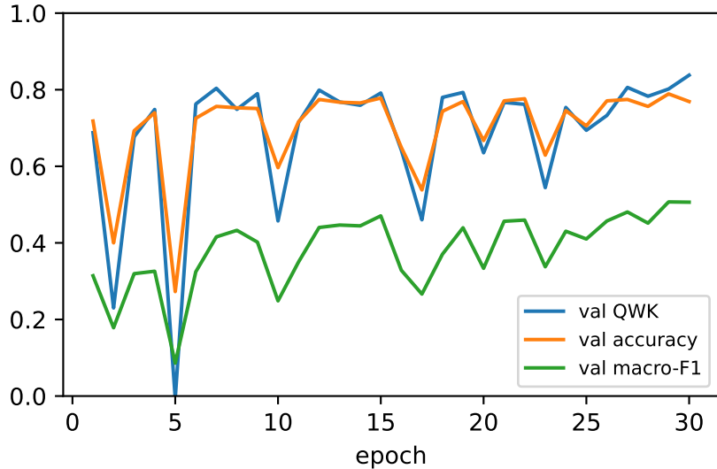
Validation metrics
