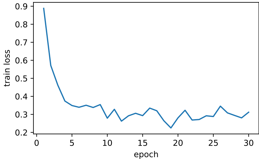
Training loss
