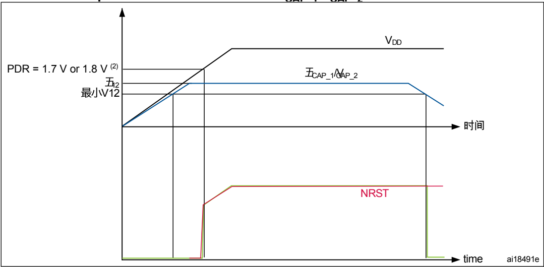
图10。在调节器关闭模式下启动：VDD斜率缓慢 - power-down reset risen after VCAP_1/VCAP_2 stabilization
