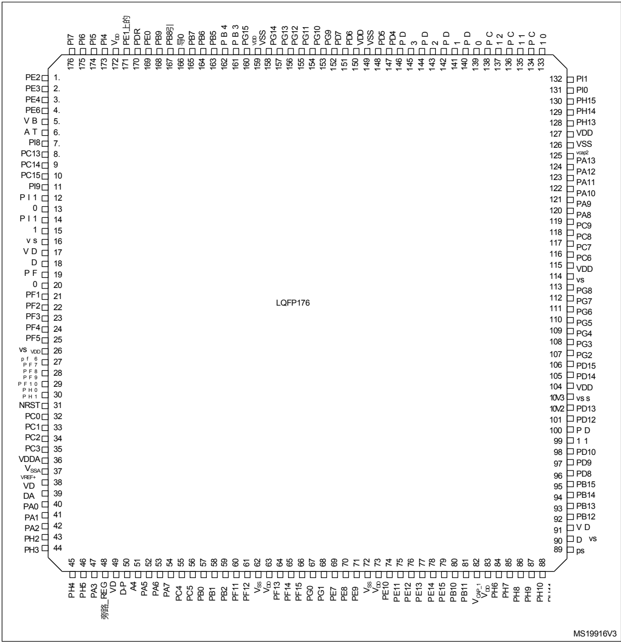
图15. STM32F40x LQFP176引脚
