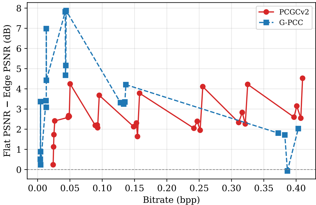
Oversmoothing Gap: PCGCv2 vs. G-PCC (avg. 4 sequences)
