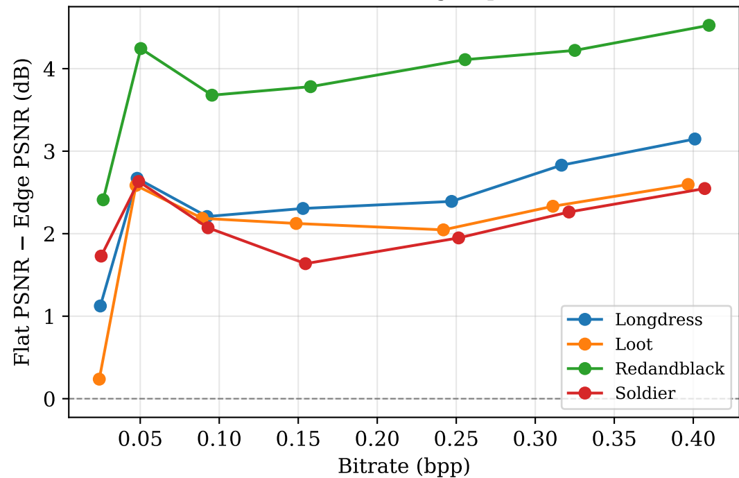
PCGCv2 Oversmoothing Gap vs. Bitrate
