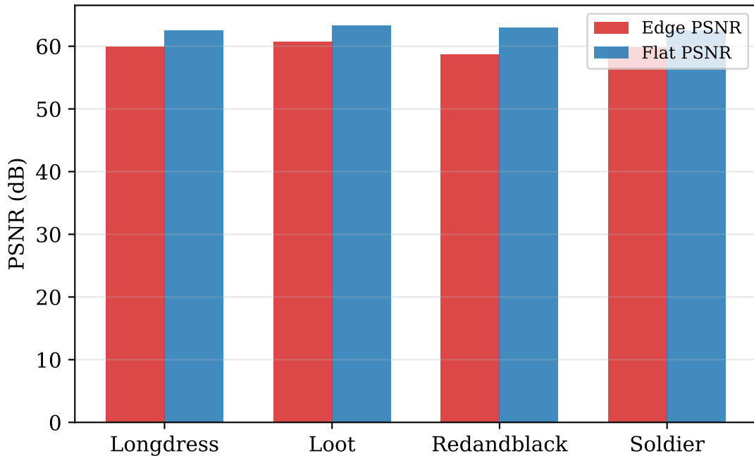
PCGCv2 Stratified PSNR at r2 (0.05 bpp)
