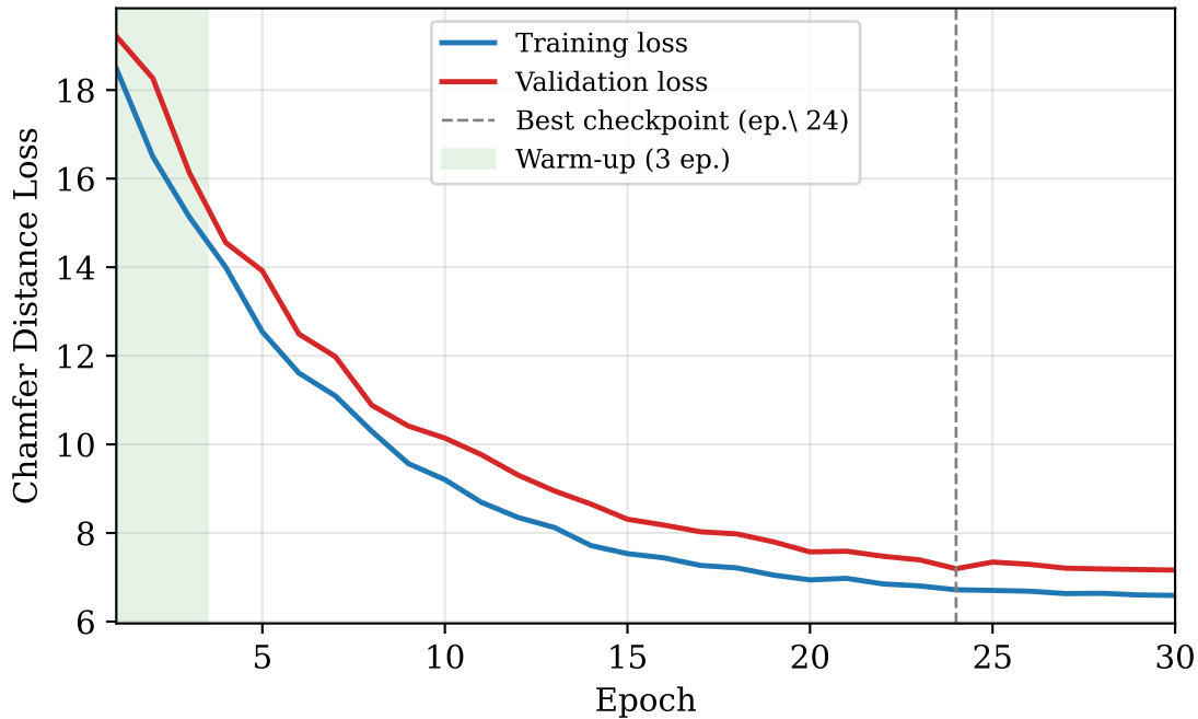
Training Curve --- v10-nocurv Model
