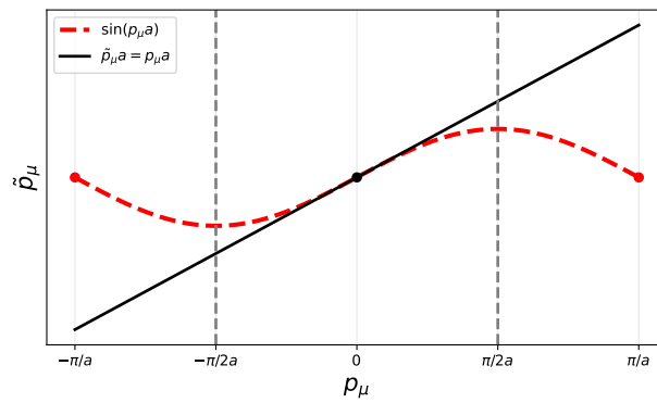
Figure 3: The effect of staggering the spinor degrees of freedom across the lattice to get an effect lattice spacing of 2a , thus halving the Brillouin zone – shown by the dashed grey line.
