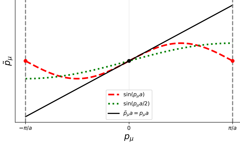
Figure 1: This is an illustration to show the effect of the missing factor of one-half from the fermion lattice momenta in Eq. (37) as opposed to case of the scalar field in Eq. (44) from lecture 1. The fermionic lattice momentum has zeros at the edges of the Brillouin zone!
