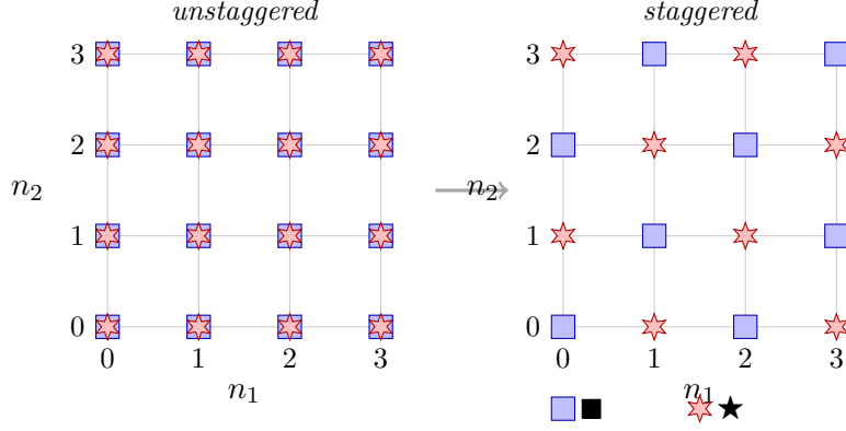
Figure 4: Left: untagged lattice — every site carries all spinor components (both \blacksquare and \star overlap). Right: staggered lattice — spinor components are distributed across sites according to the parity of n_1 + n_2 , effectively doubling the lattice spacing.
