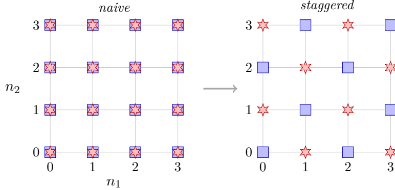
Figure 4: Assuming that we have a two-component spinor at each lattice site, given by a square and a star. On the left: naive lattice with lattice spacing a , and every site carries all spinor components. On the right: staggered lattice – spinor components are distributed across sites, effectively doubling the lattice spacing.
