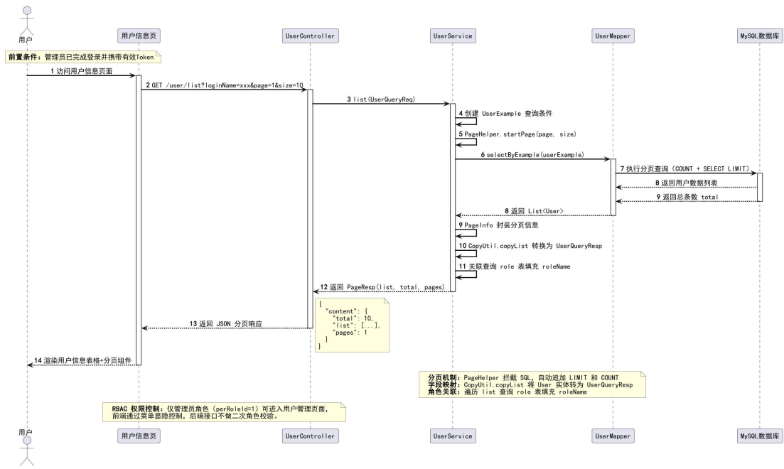
Figure 4.5 User Info Sequence Diagram
