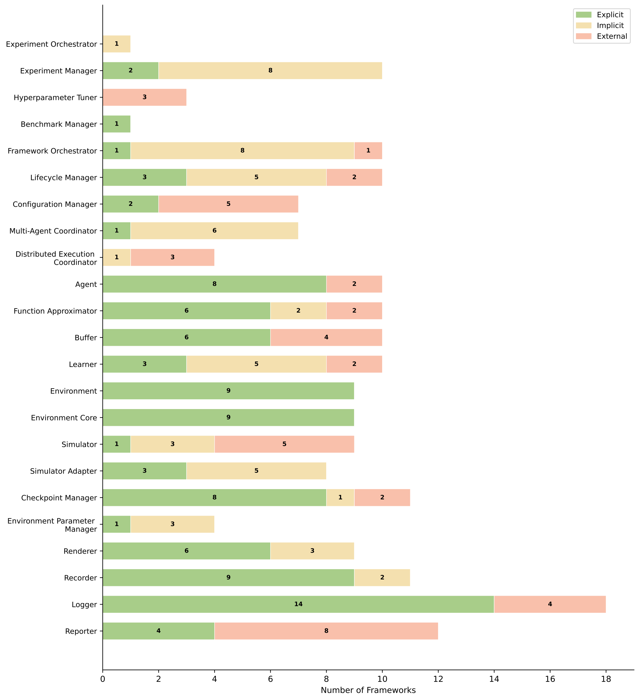
Implementation Status of Components across Analyzed RL Frameworks
