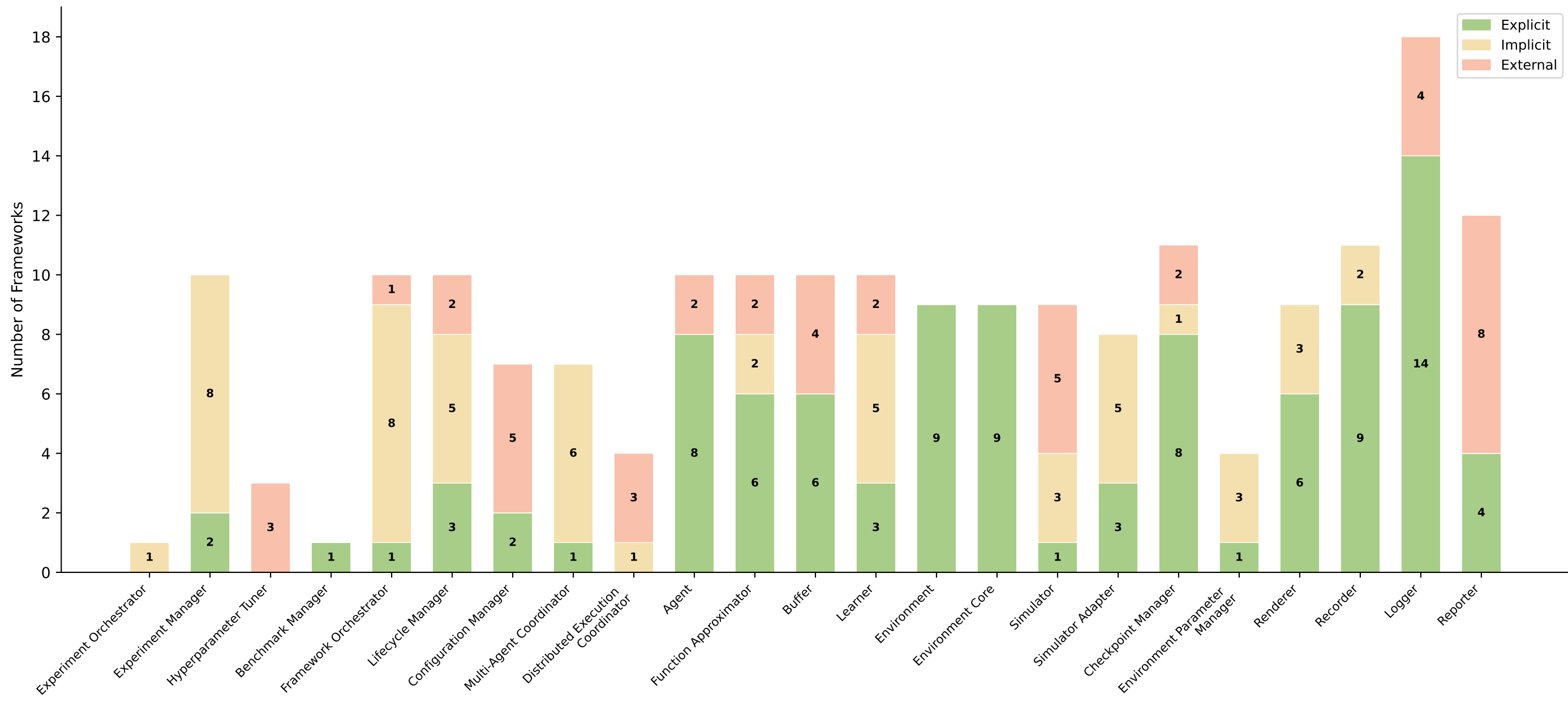
Implementation Status of Components across Analyzed RL Frameworks
