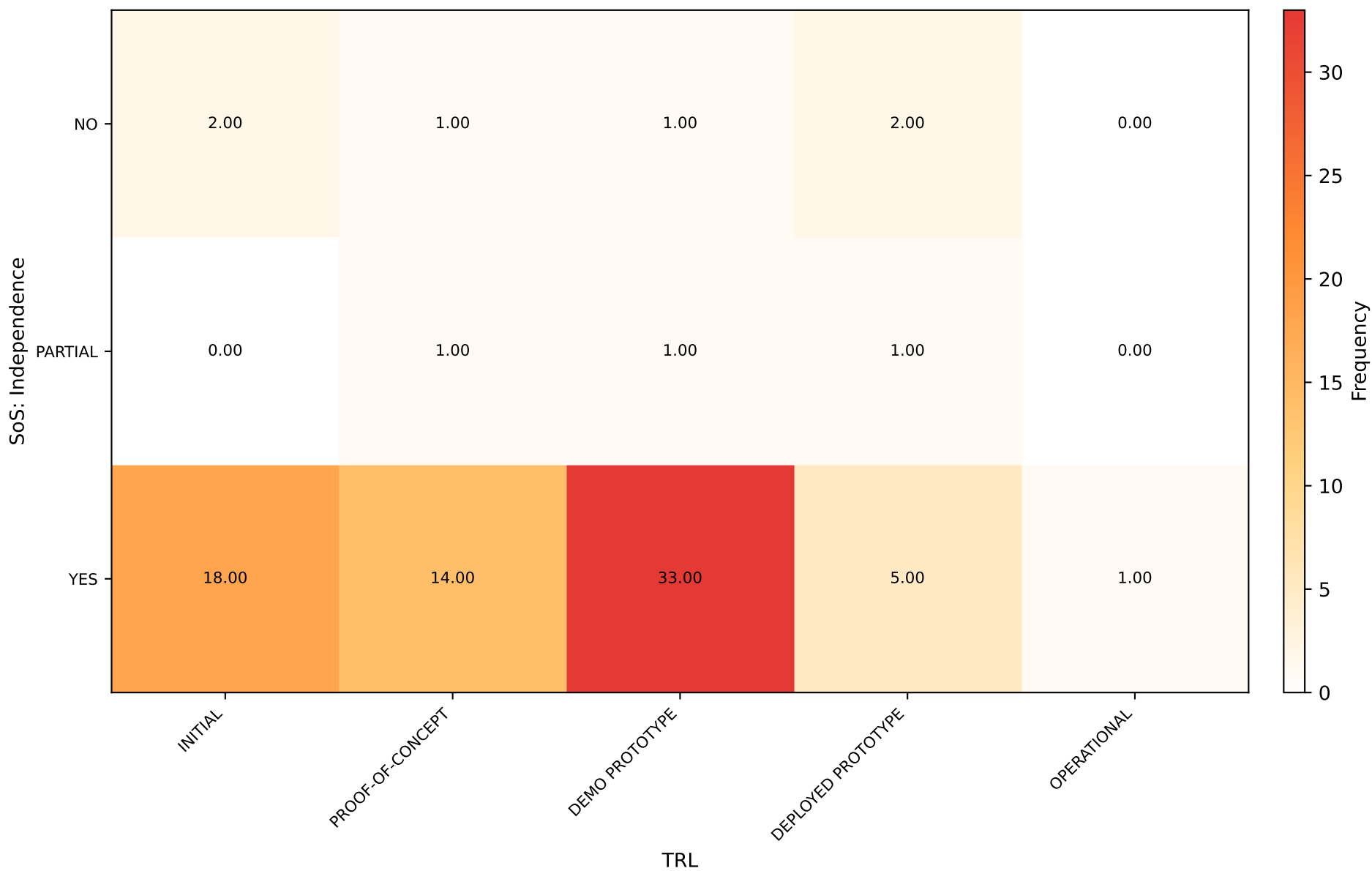
SoS: Independence vs TRL [NO] ( \chi^2=8.072 , p=0.4265 )
