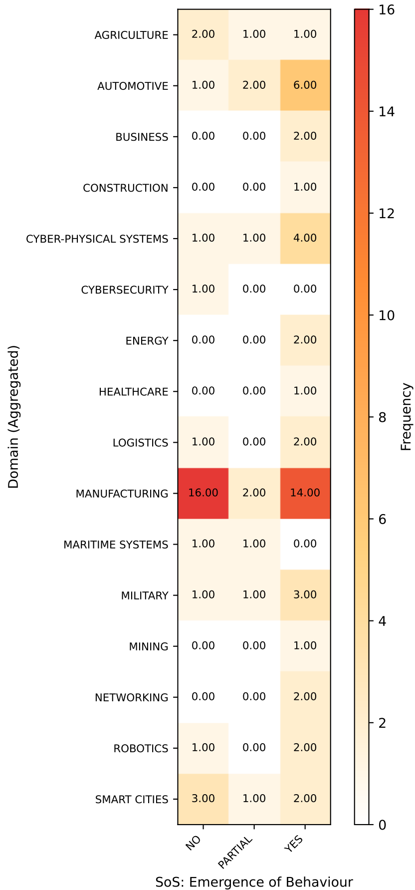
Domain (Aggregated) vs SoS: Emergence of Behaviour [NO] ( \chi^2=24.583 , p=0.745 )
