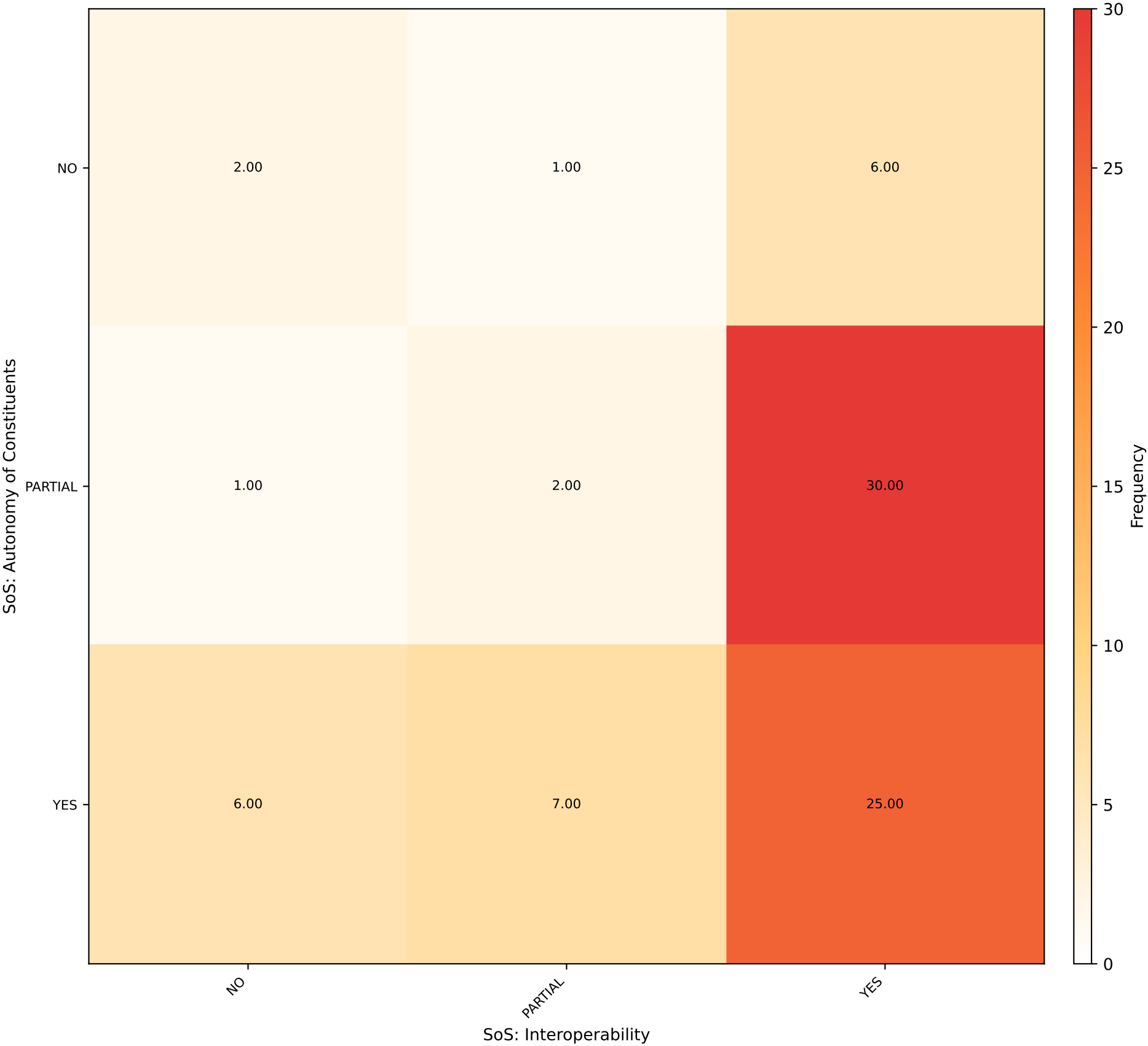
SoS: Autonomy of Constituents vs SoS: Interoperability [NO] (chi²=7.399, p=0.1162)
