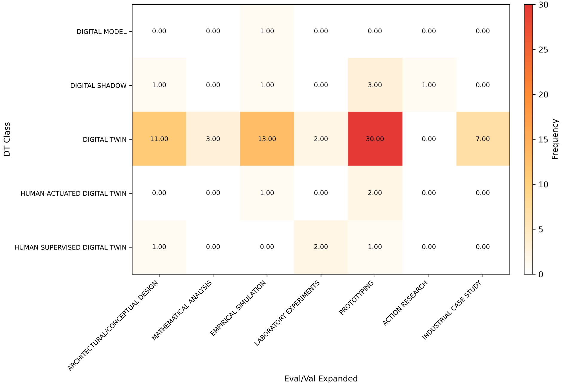
DT Class vs Eval/Val Expanded [SIG] ( \chi^2=37.971 , p=0.03491 )
