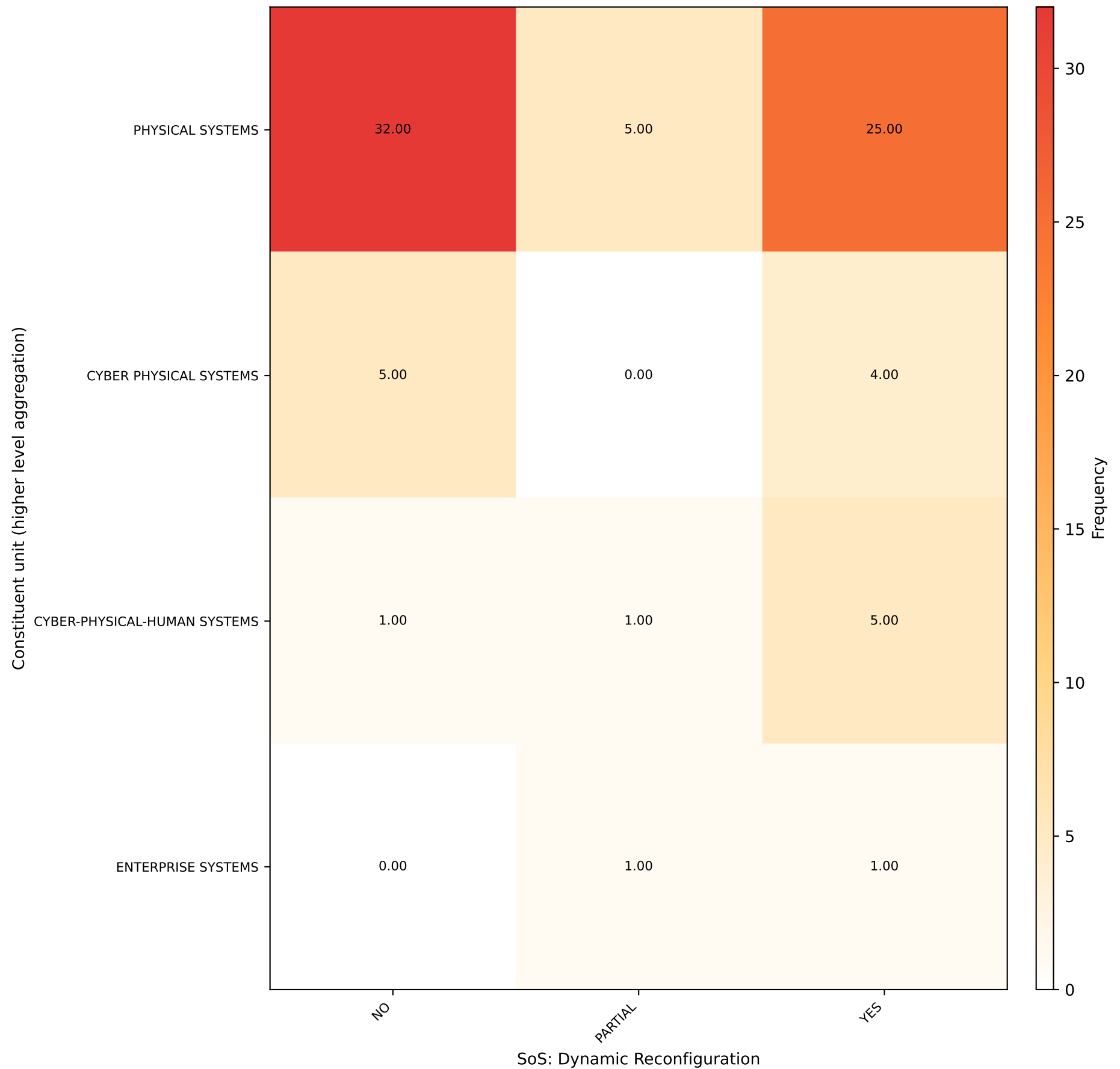
Constituent unit (higher level aggregation) vs SoS: Dynamic Reconfiguration [NO] ( \chi^2=9.286 , p=0.1581 )
