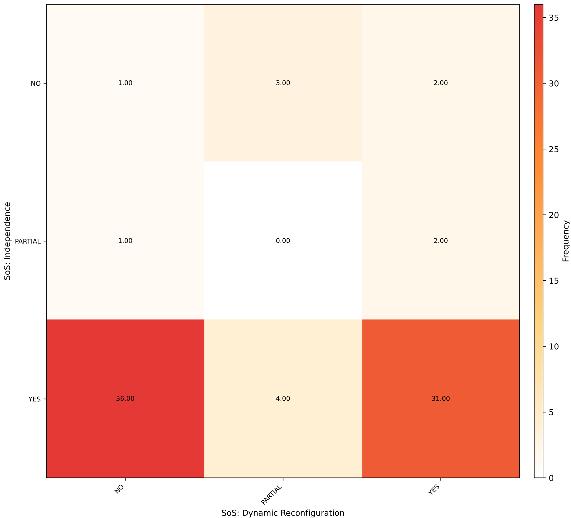
SoS: Independence vs SoS: Dynamic Reconfiguration [SIG] ( \chi^2=14.708 , p=0.005346 )
