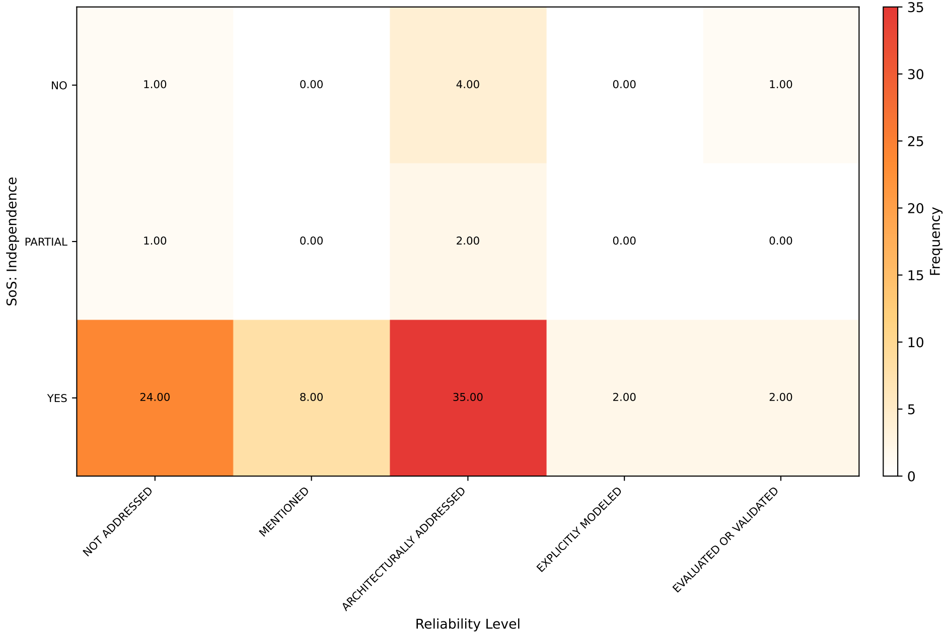
SoS: Independence vs Reliability Level [NO] ( \chi^2=5.185 , p=0.7376 )
