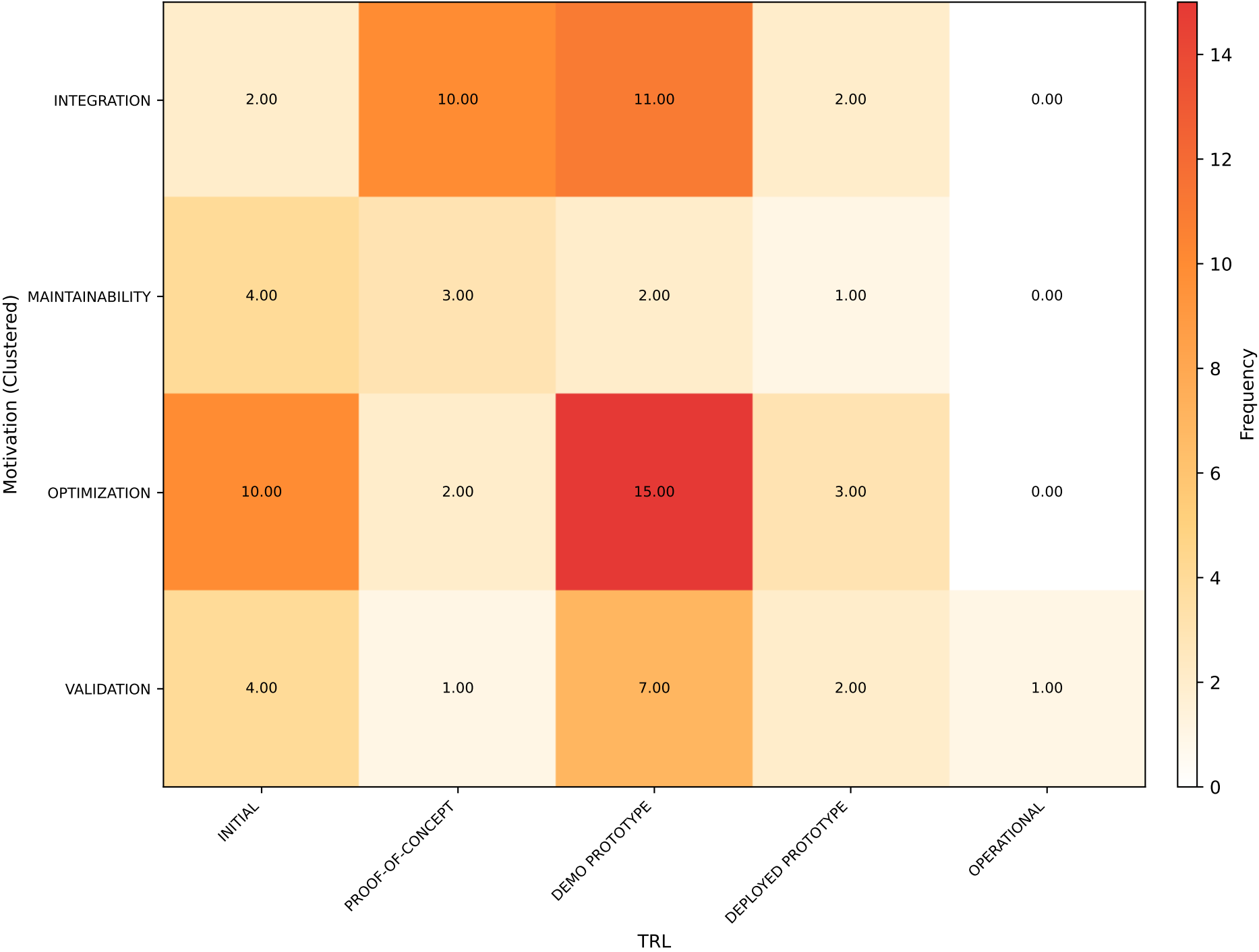
Motivation (Clustered) vs TRL [MARGINAL] (chi²=20.327, p=0.06115)
