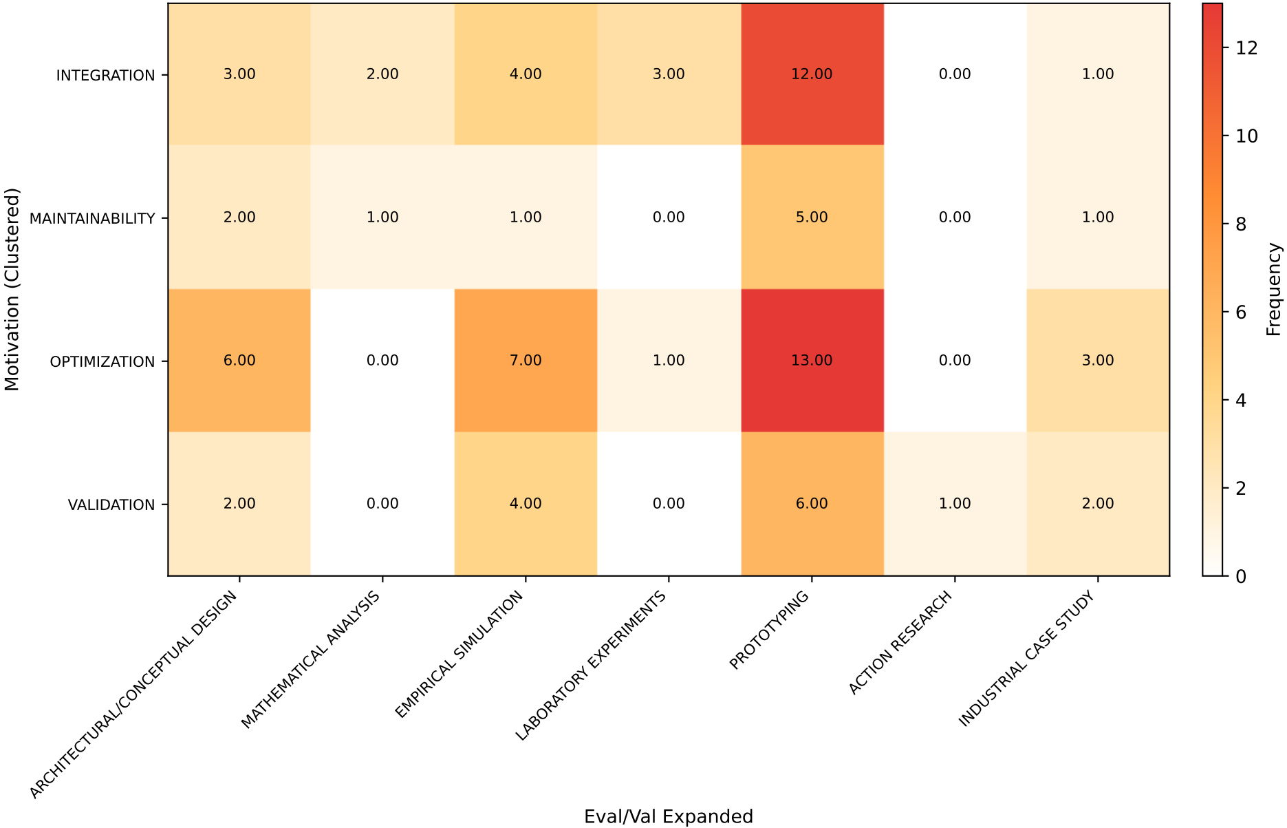
Motivation (Clustered) vs Eval/Val Expanded [NO] (chi²=15.319, p=0.6399)
