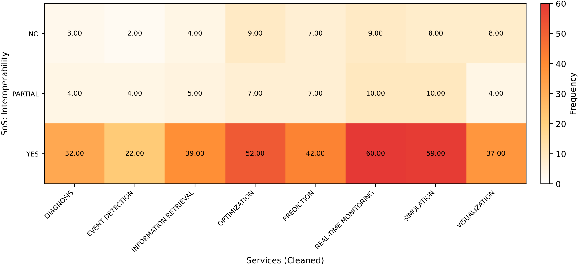
SoS: Interoperability vs Services (Cleaned) [NO] (chi²=4.155, p=0.9945)
