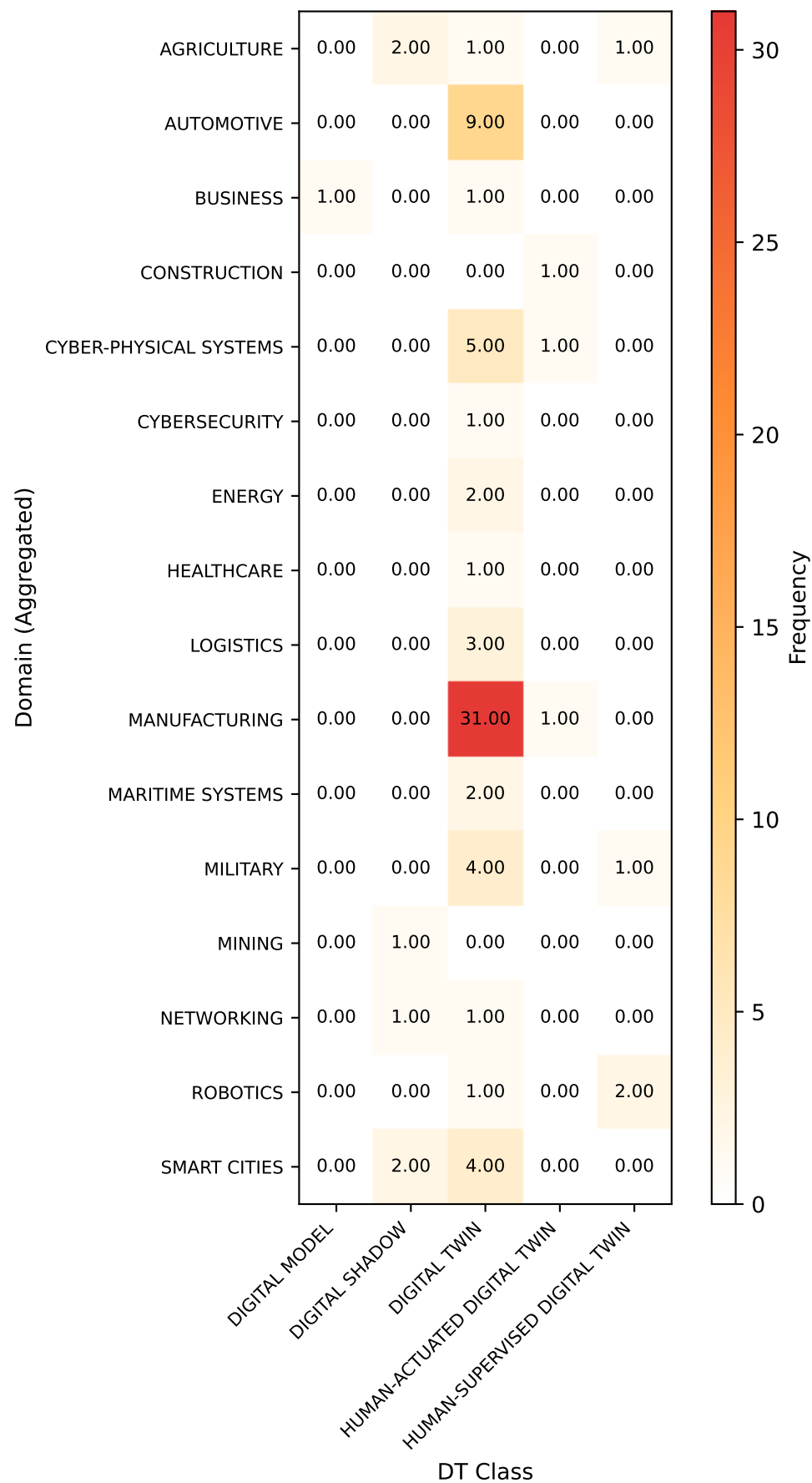
Domain (Aggregated) vs DT Class [SIG] ( \chi^2=142.134 , p=1.285e-08 )
