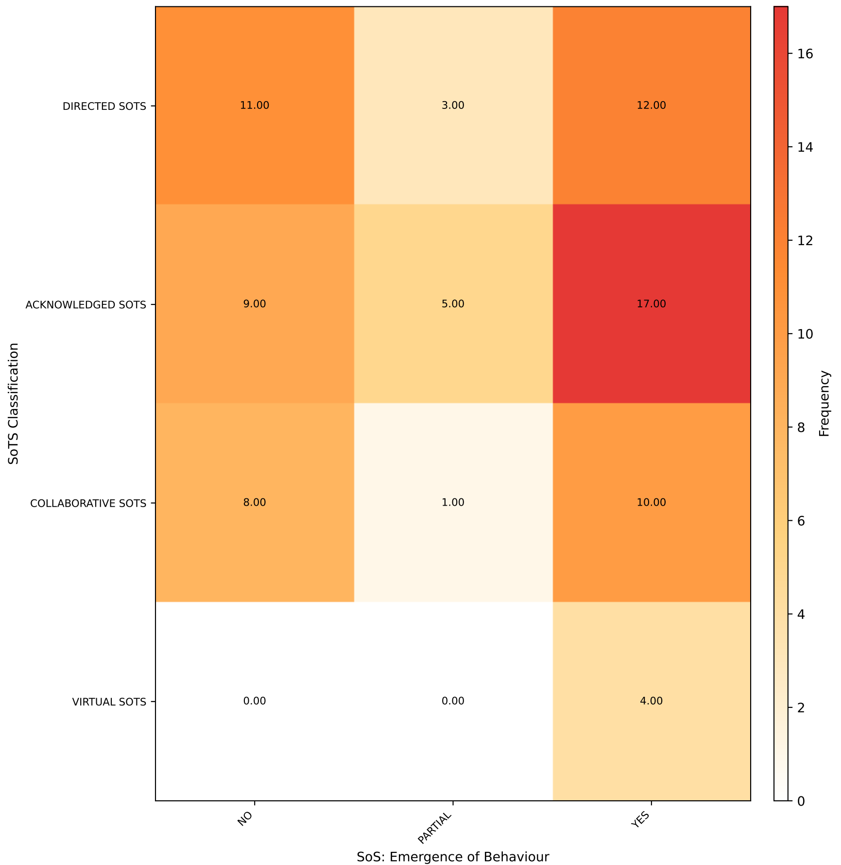
SoTS Classification vs SoS: Emergence of Behaviour [NO] ( \chi^2=5.982 , p=0.4252 )
