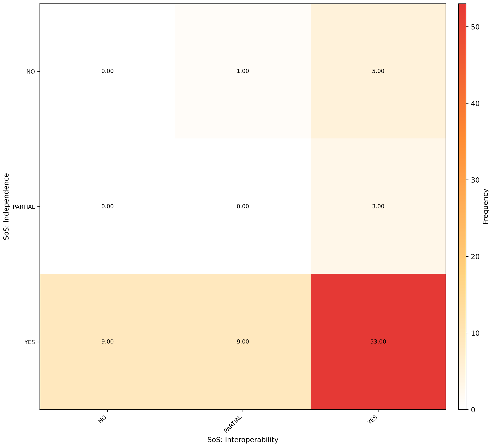
SoS: Independence vs SoS: Interoperability [NO] ( \chi^2=1.886 , p=0.7567 )
