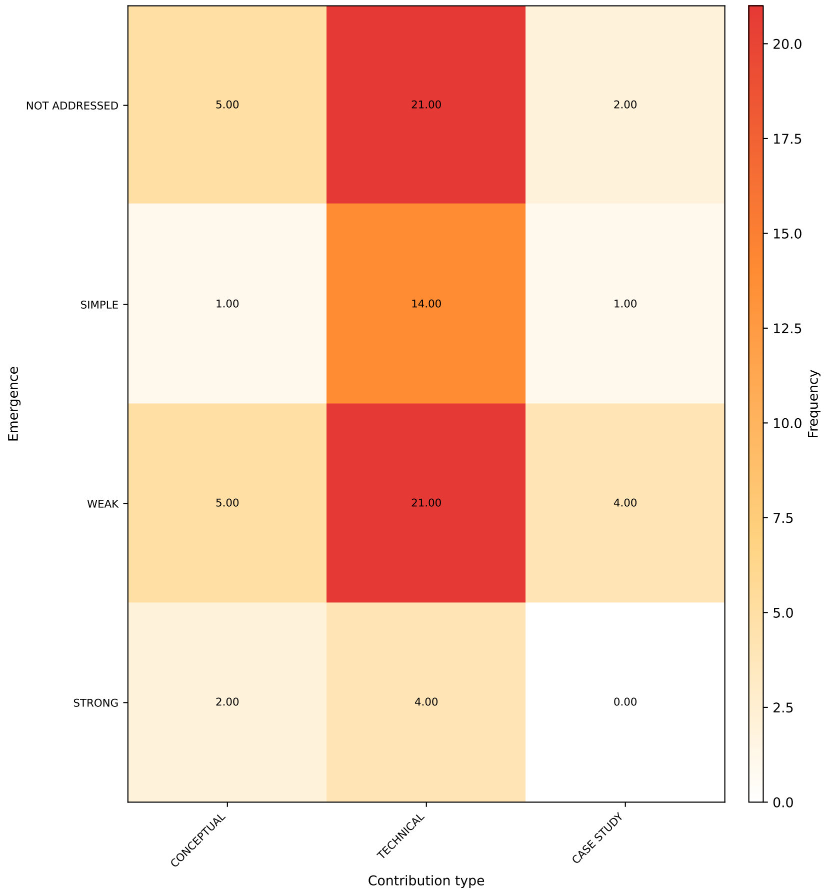
Emergence vs Contribution type [NO] ( \chi^2=4.041 , p=0.6711 )
