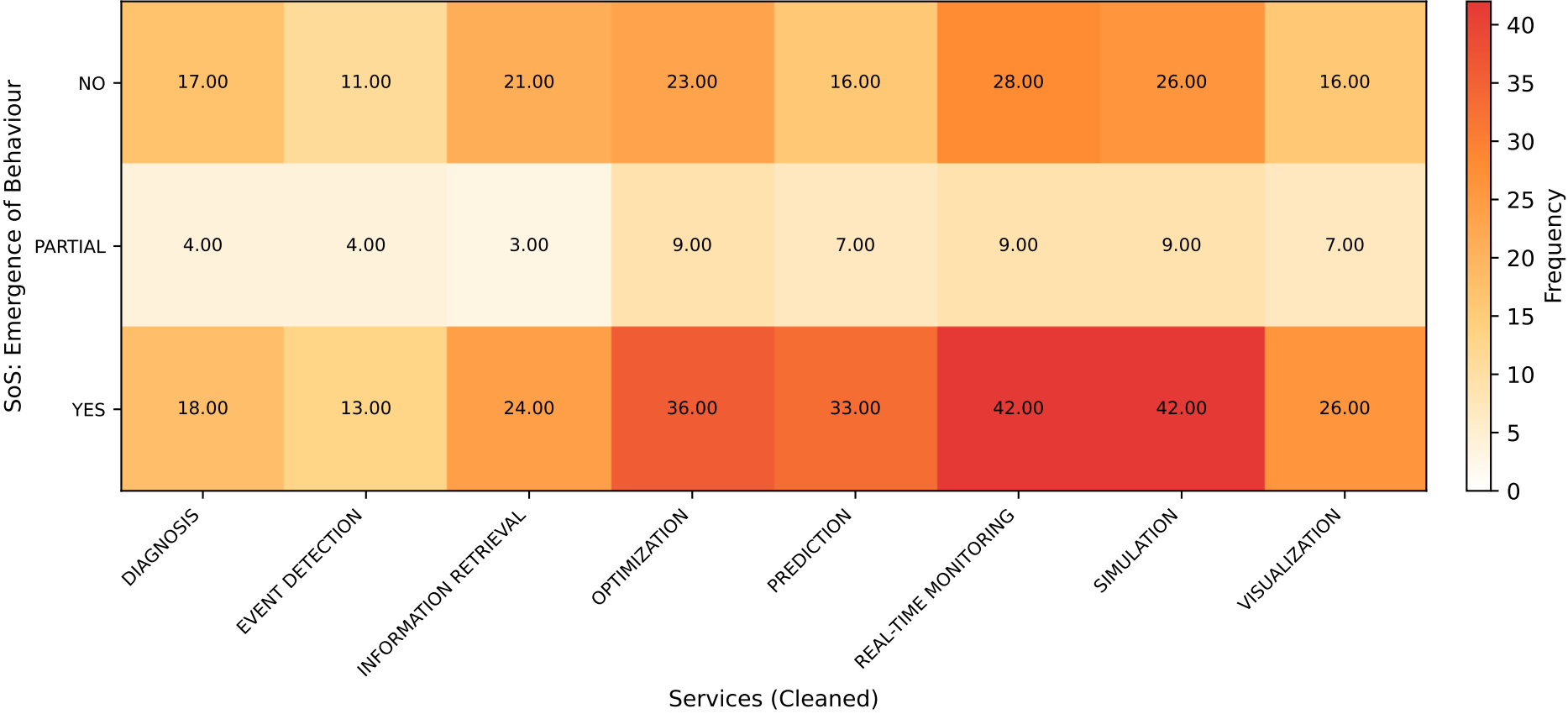
SoS: Emergence of Behaviour vs Services (Cleaned) [NO] (chi²=5.693, p=0.9737)
