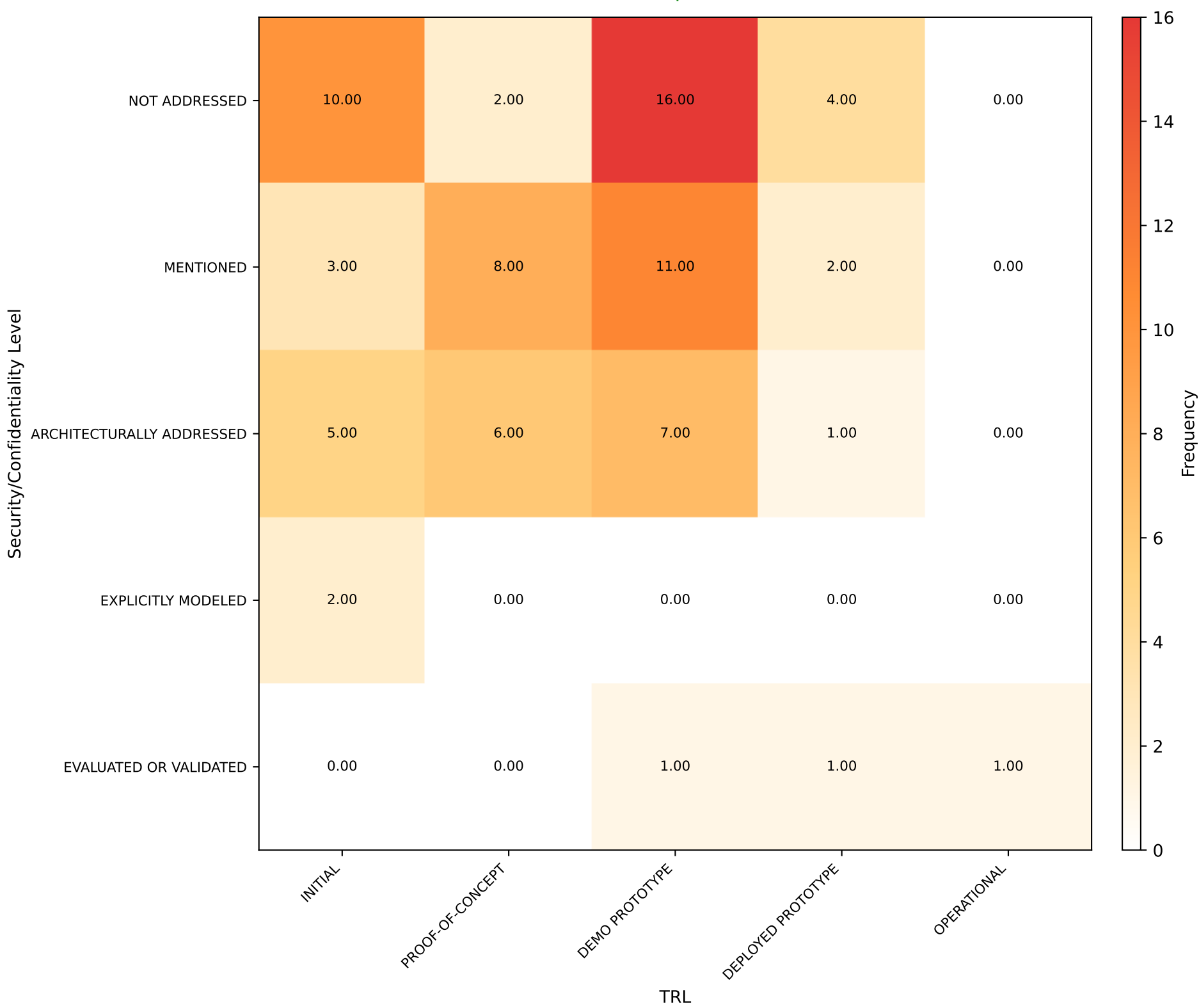
Security/Confidentiality Level vs TRL [SIG] ( \chi^2=44.354 , p=0.0001742 )
