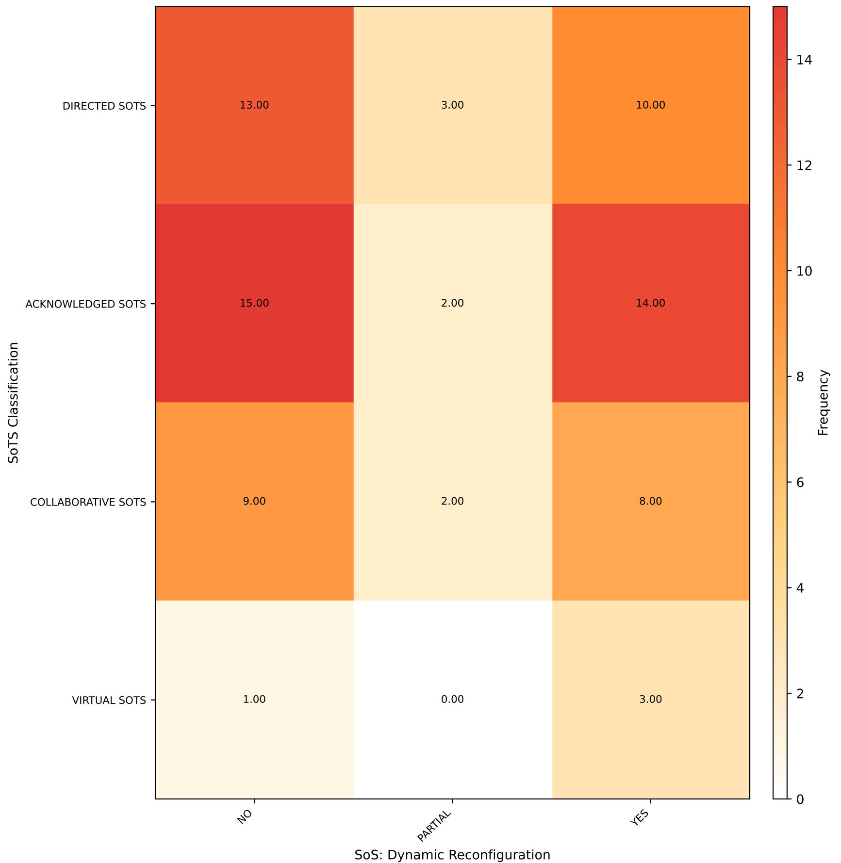
SoTS Classification vs SoS: Dynamic Reconfiguration [NO] ( \chi^2=2.387 , p=0.8809 )
