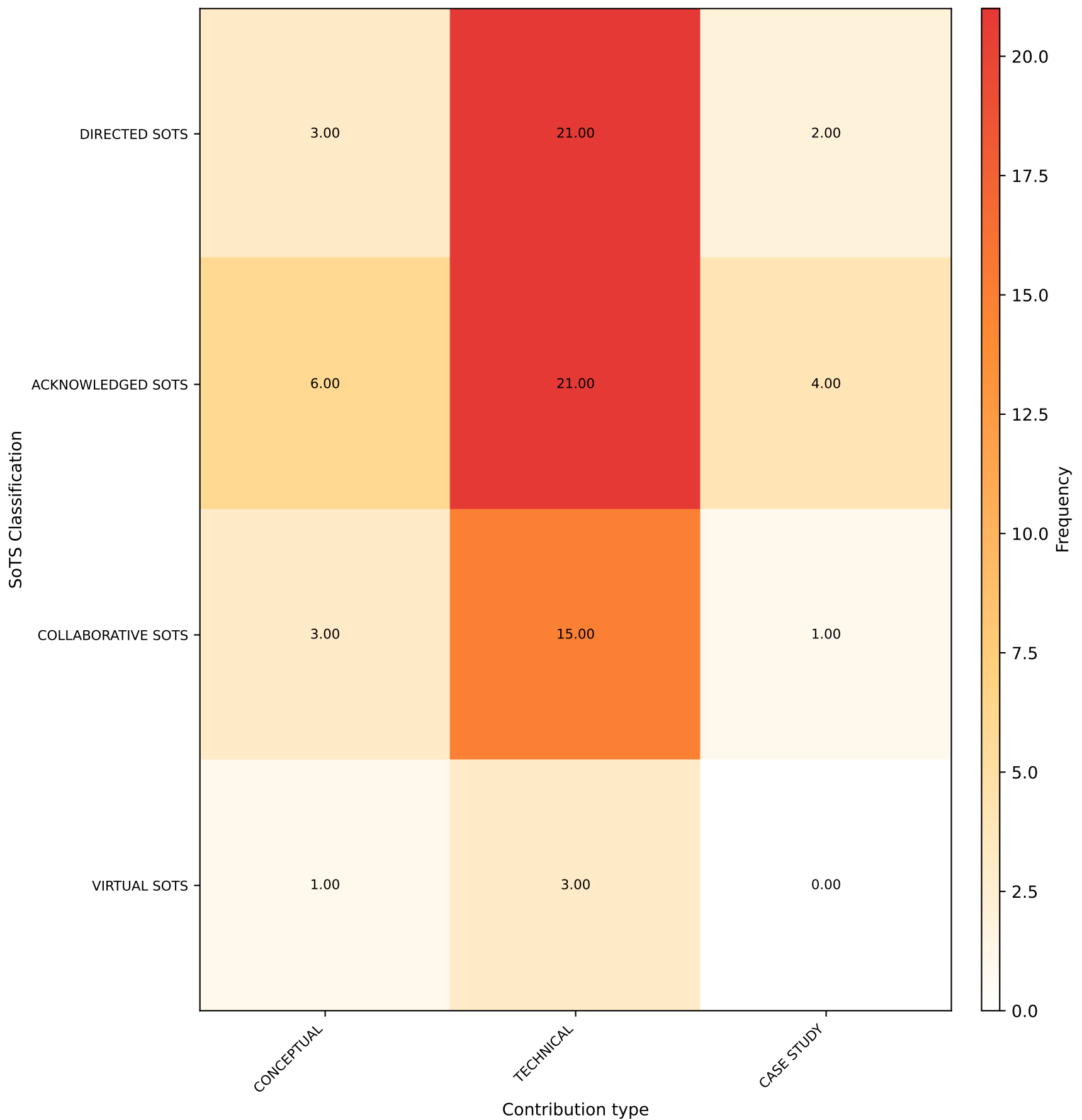
SoTS Classification vs Contribution type [NO] ( \chi^2=2.361 , p=0.8837 )
