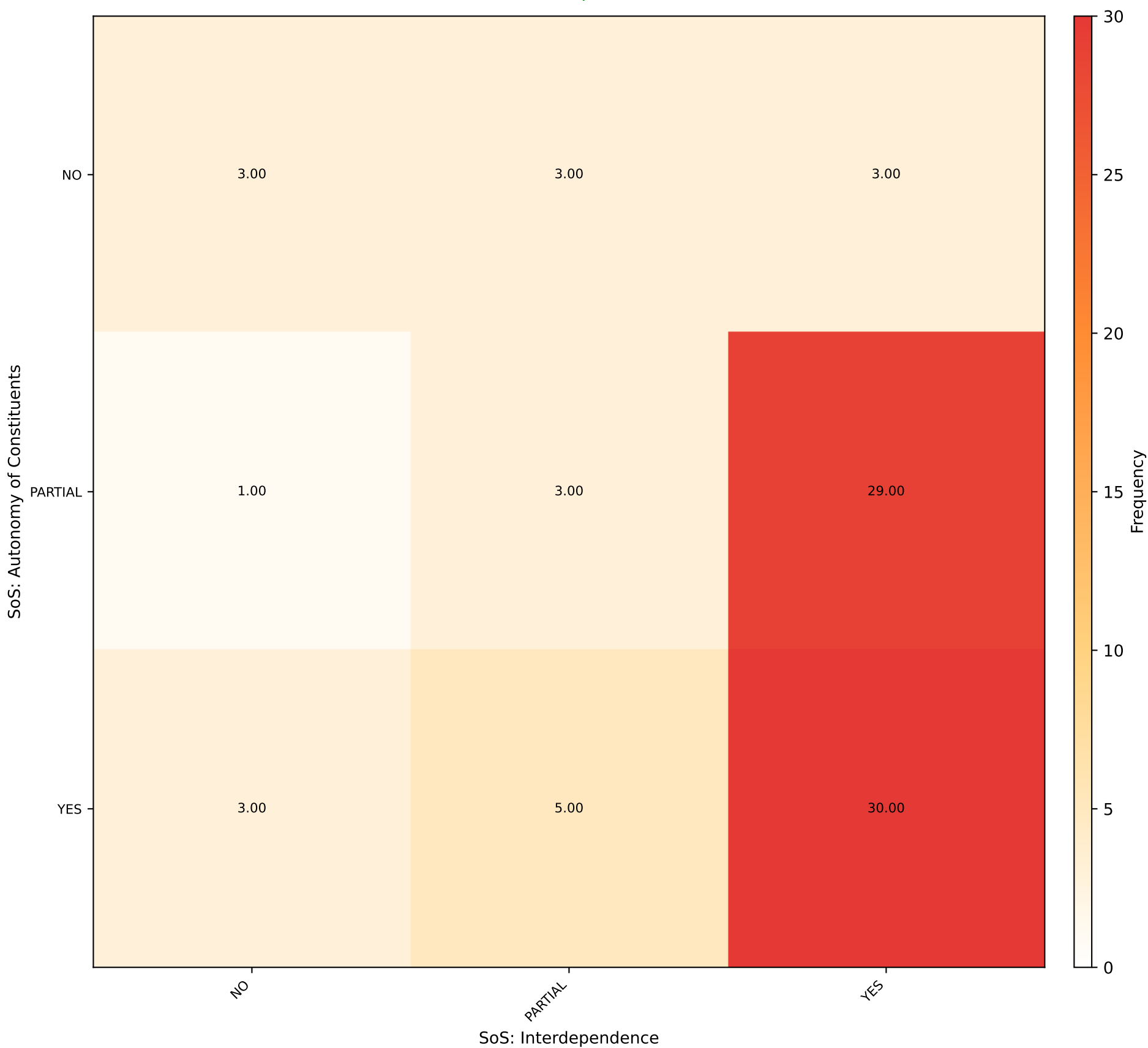
SoS: Autonomy of Constituents vs SoS: Interdependence [SIG] ( \chi^2=13.257 , p=0.01009 )
