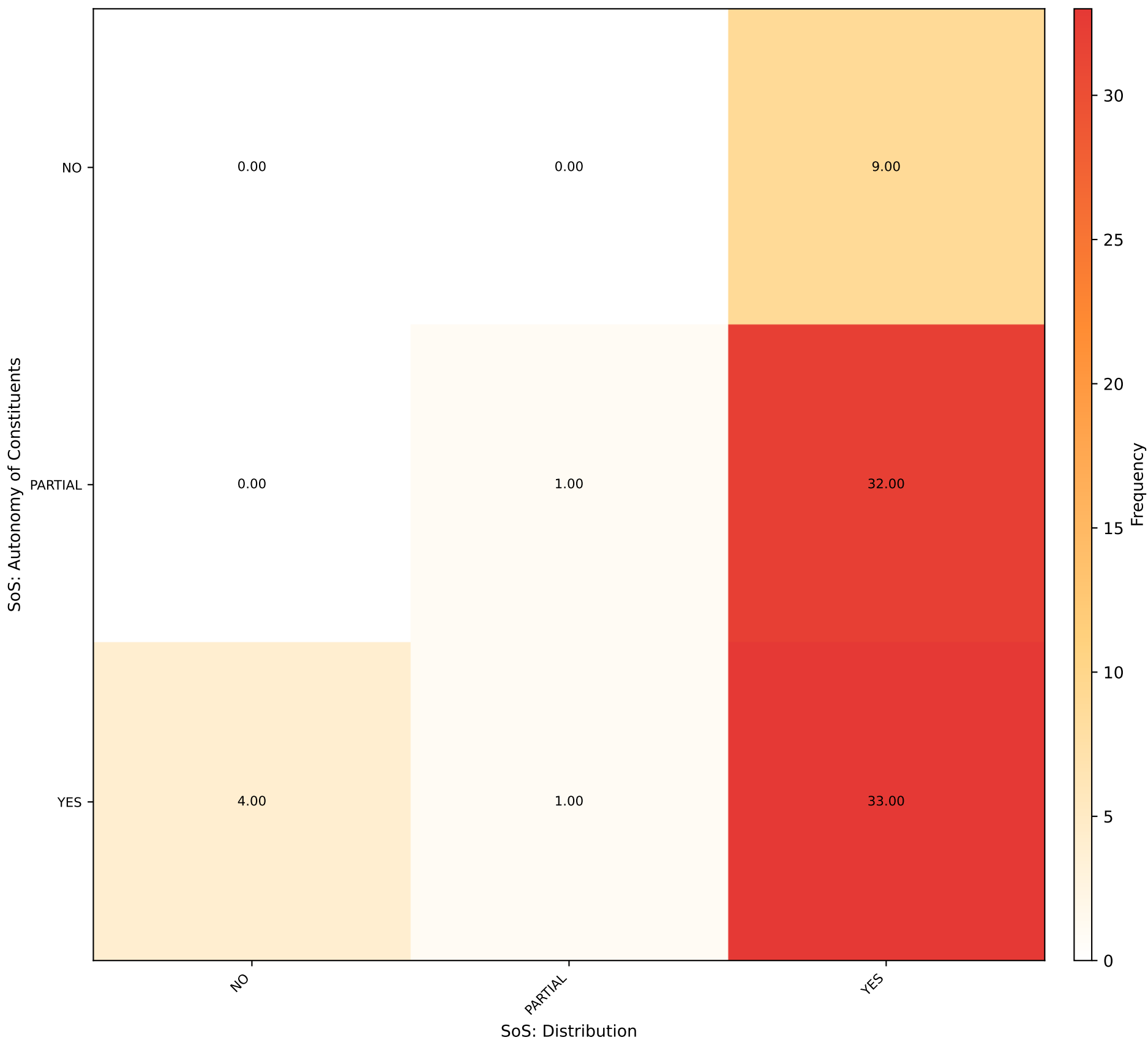
SoS: Autonomy of Constituents vs SoS: Distribution [NO] ( \chi^2=4.943 , p=0.2932 )
