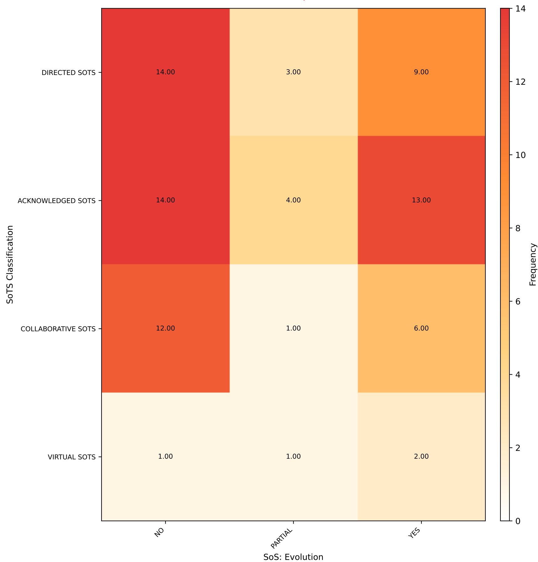
SoTS Classification vs SoS: Evolution [NO] (chi²=3.241, p=0.778)
