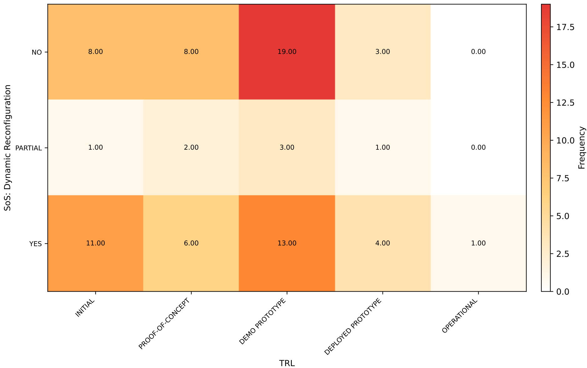
SoS: Dynamic Reconfiguration vs TRL [NO] ( \chi^2=3.902 , p=0.8659 )
