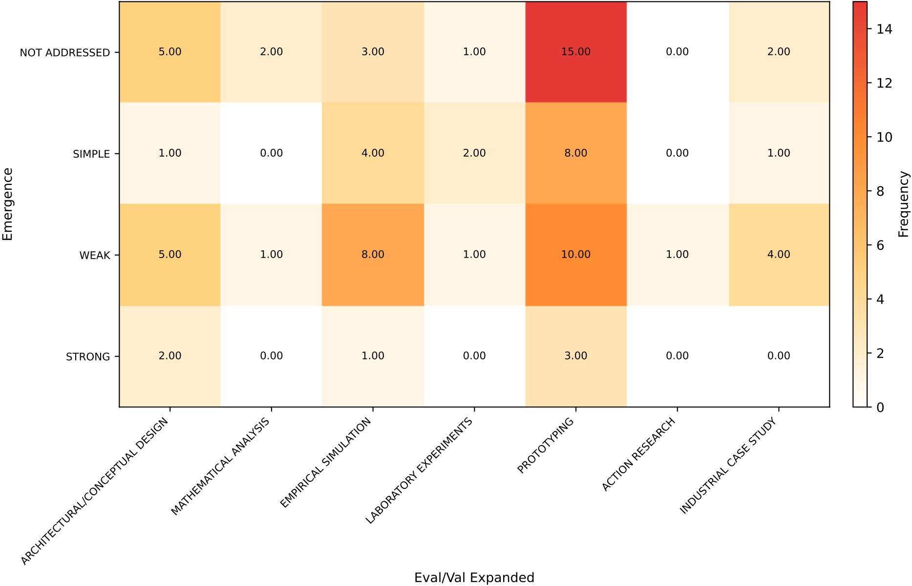
Emergence vs Eval/Val Expanded [NO] (chi²=12.892, p=0.7979)
