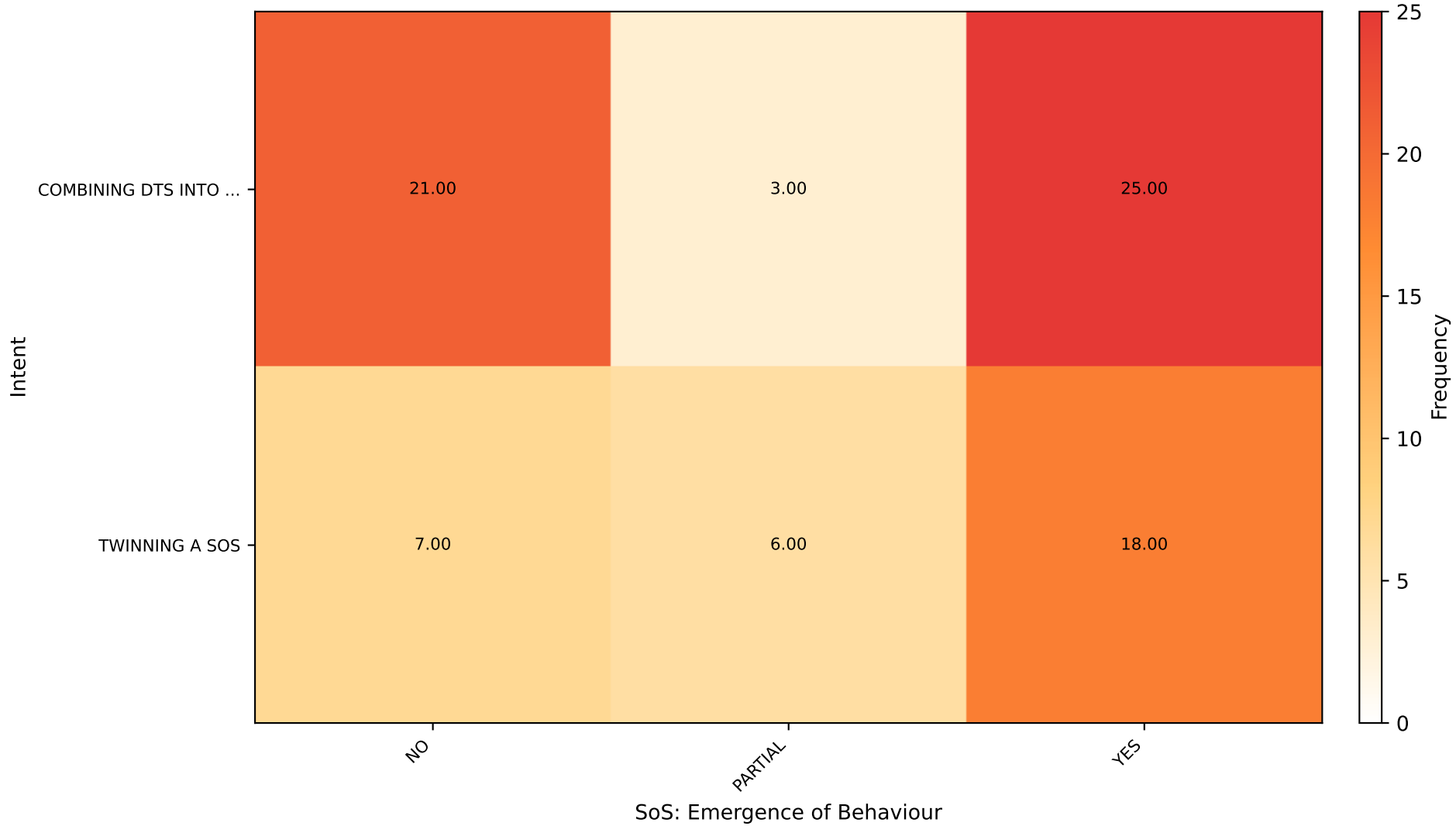
Intent vs SoS: Emergence of Behaviour [MARGINAL] ( \chi^2=5.361 , p=0.06853 )
