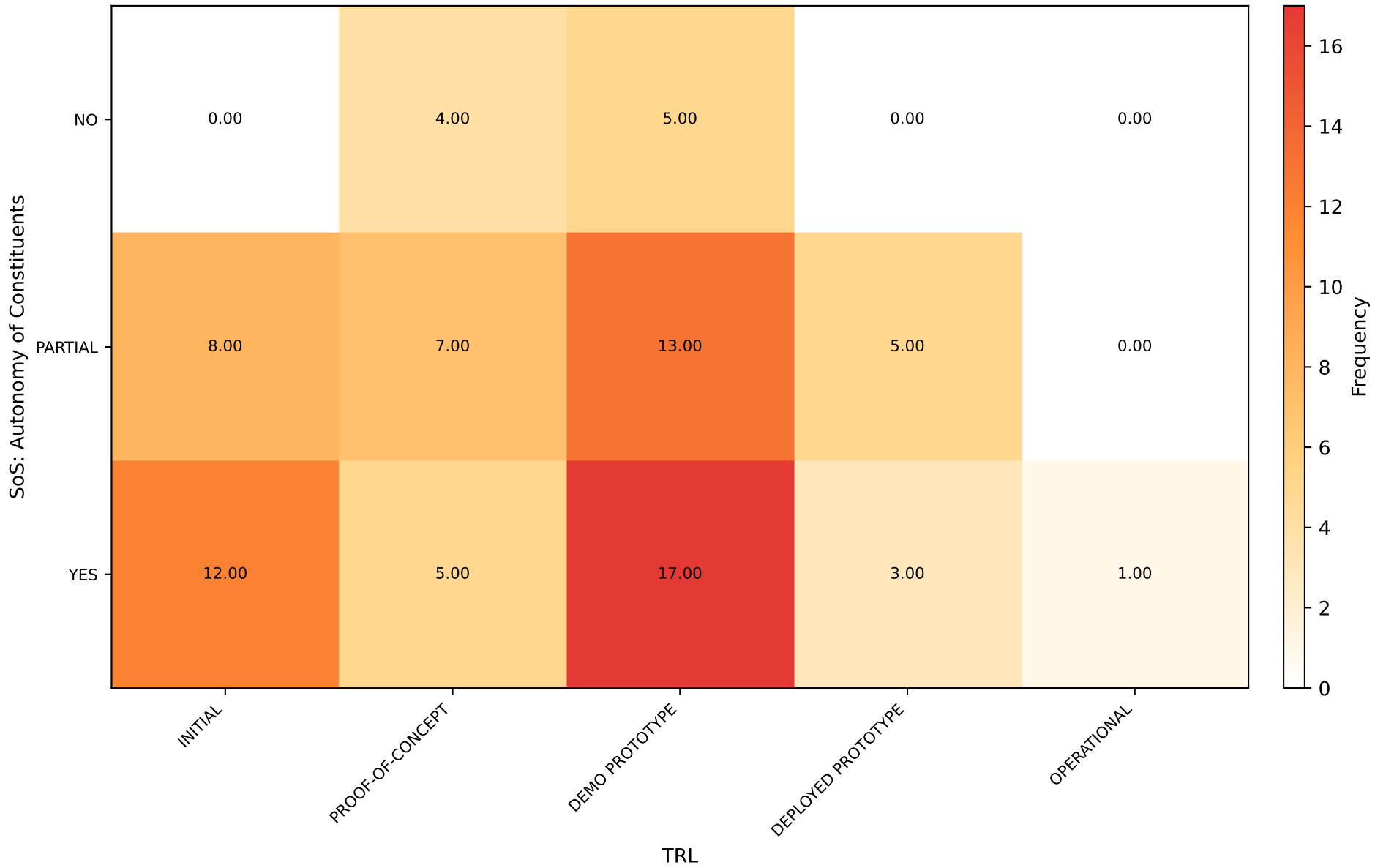
SoS: Autonomy of Constituents vs TRL [NO] ( \chi^2=10.006 , p=0.2646 )
