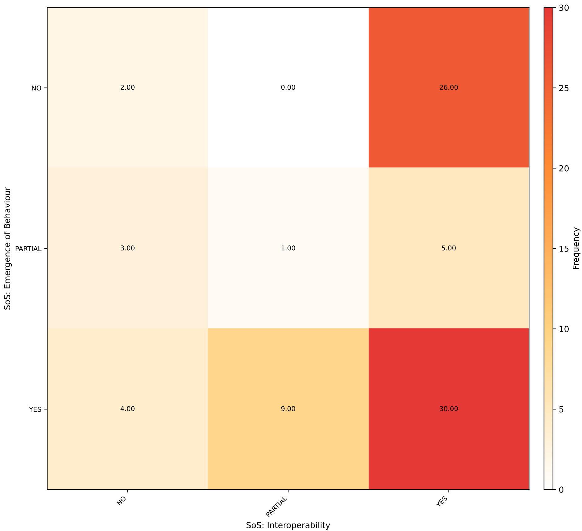
SoS: Emergence of Behaviour vs SoS: Interoperability [SIG] ( \chi^2=12.180 , p=0.01606 )
