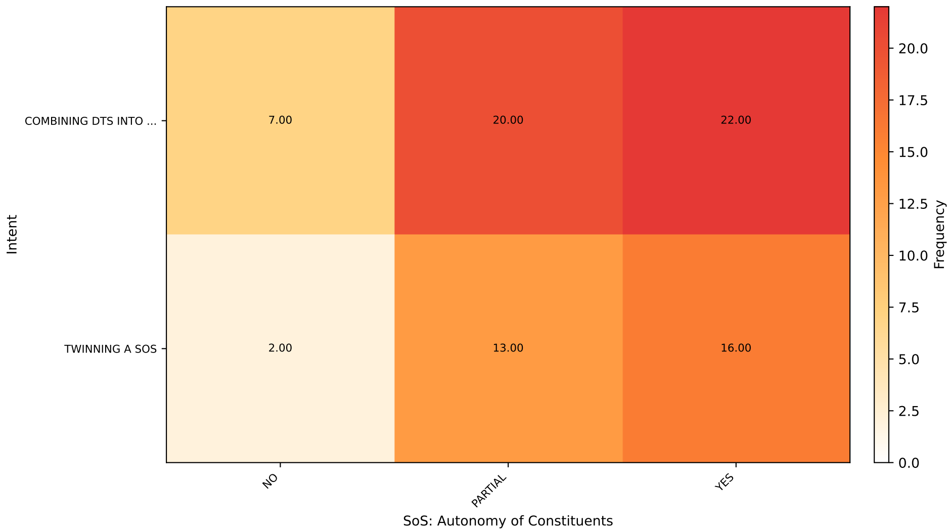
Intent vs SoS: Autonomy of Constituents [NO] ( \chi^2=1.222 , p=0.5428 )
