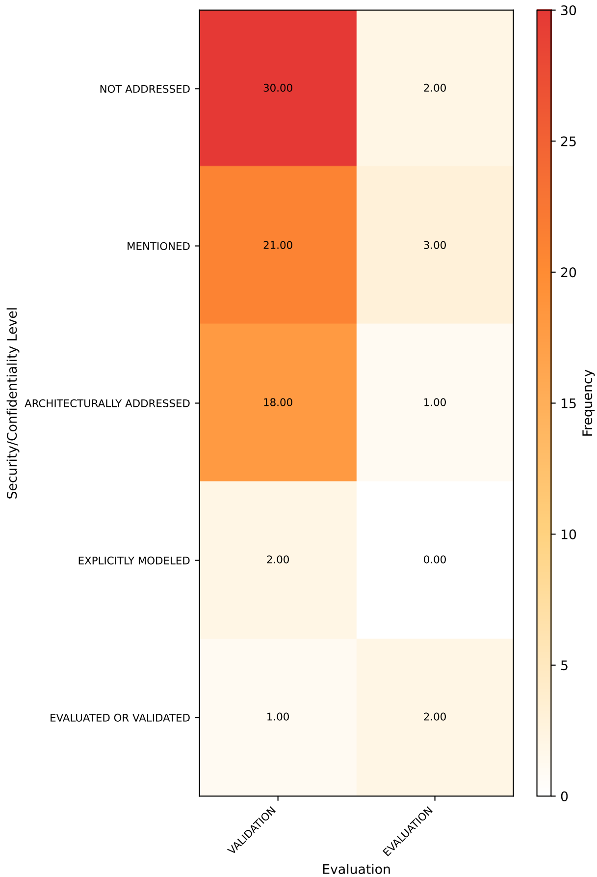
Security/Confidentiality Level vs Evaluation [SIG] ( \chi^2=12.066 , p=0.01687 )
