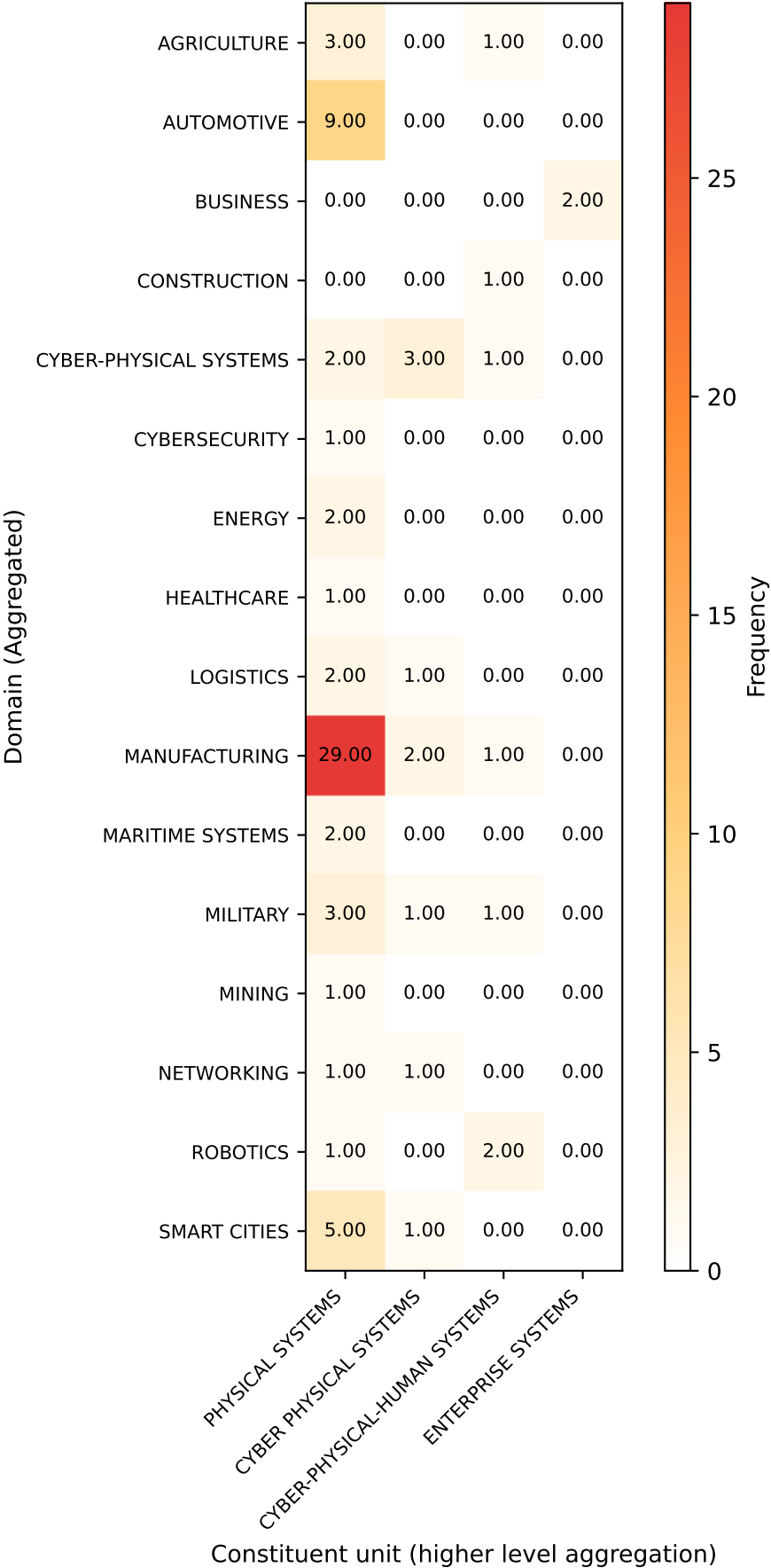
Domain (Aggregated) vs Constituent unit (higher level aggregation) [SIG] (chi²=127.997, p=6.829e-10)
