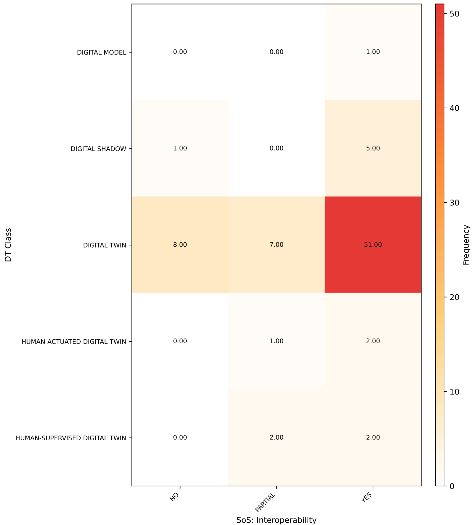
DT Class vs SoS: Interoperability [NO] ( \chi^2=8.227 , p=0.4116 )
