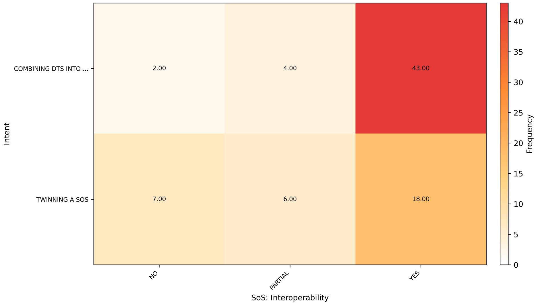
Intent vs SoS: Interoperability [SIG] ( \chi^2=9.874 , p=0.007178 )
