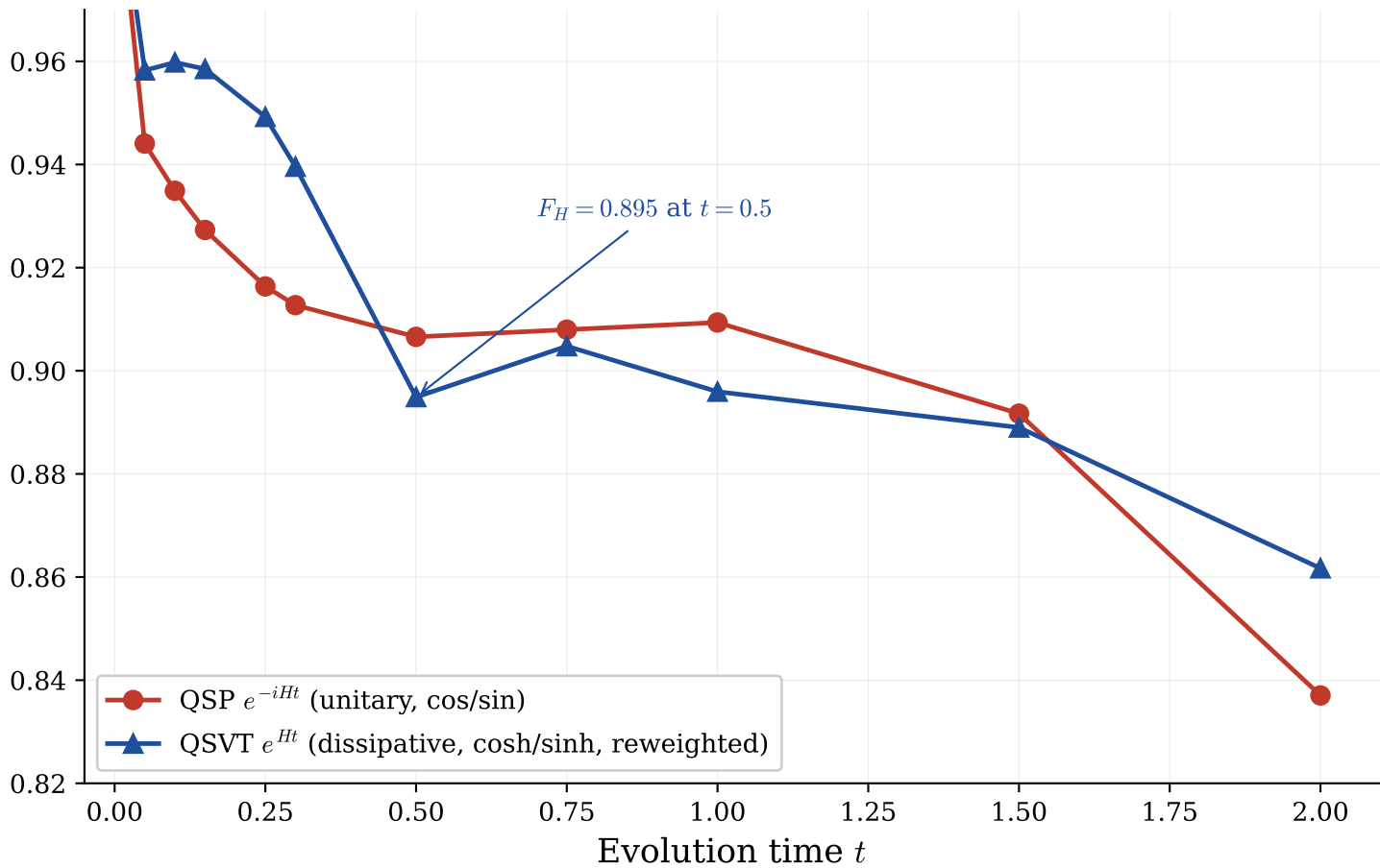
Hellinger fidelity F_H vs CTMC
