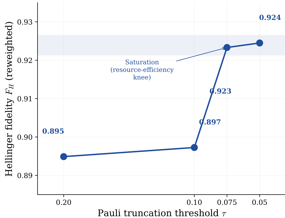
Monotone-saturating fidelity under Pauli truncation ( t = 0.5 , corrected pipeline)
