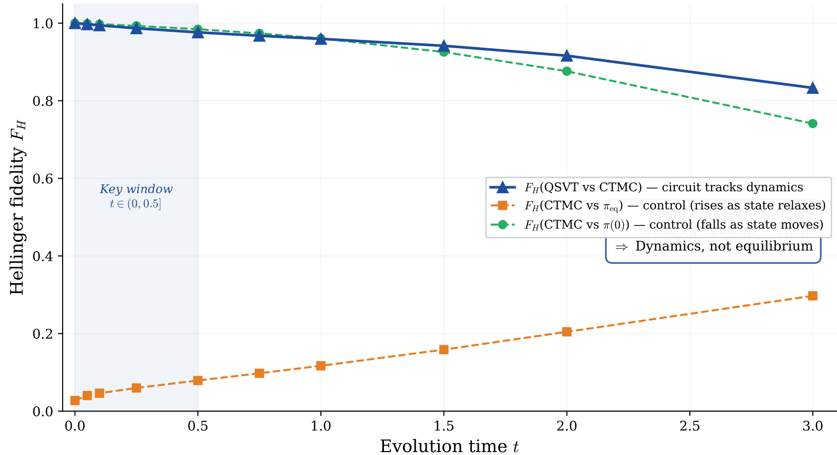
Far-from-equilibrium QSVT trajectory (delta start on delta on least-frequent codon ACG, F_H(\pi(0), \pi_{\text{eq}}) = 0.027 )
