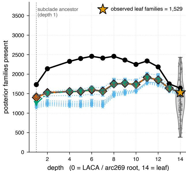
posterior families present per node (uncorrected)
