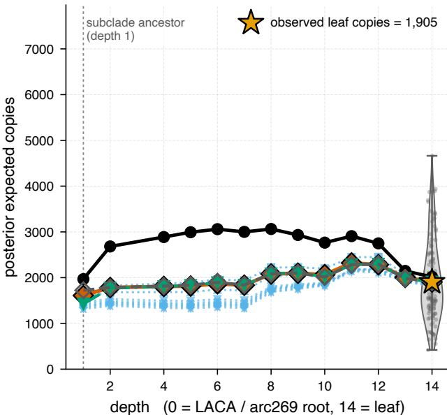
posterior copies per node (uncorrected)
