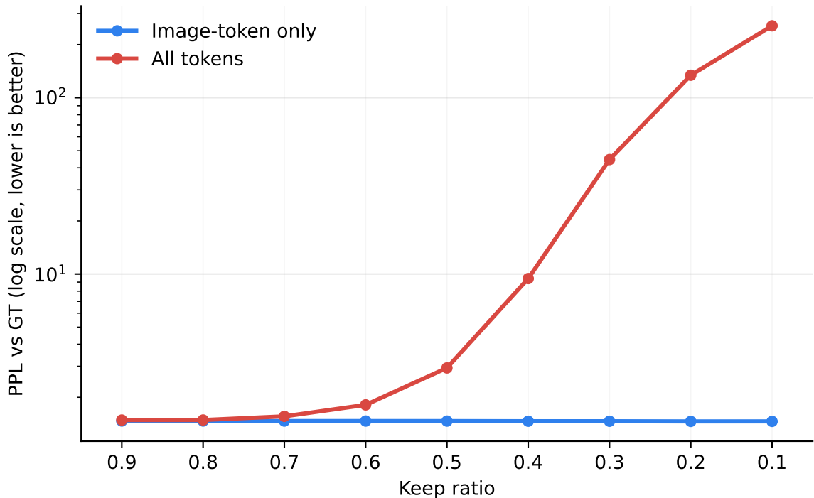
DocVQA random eviction: PPL
