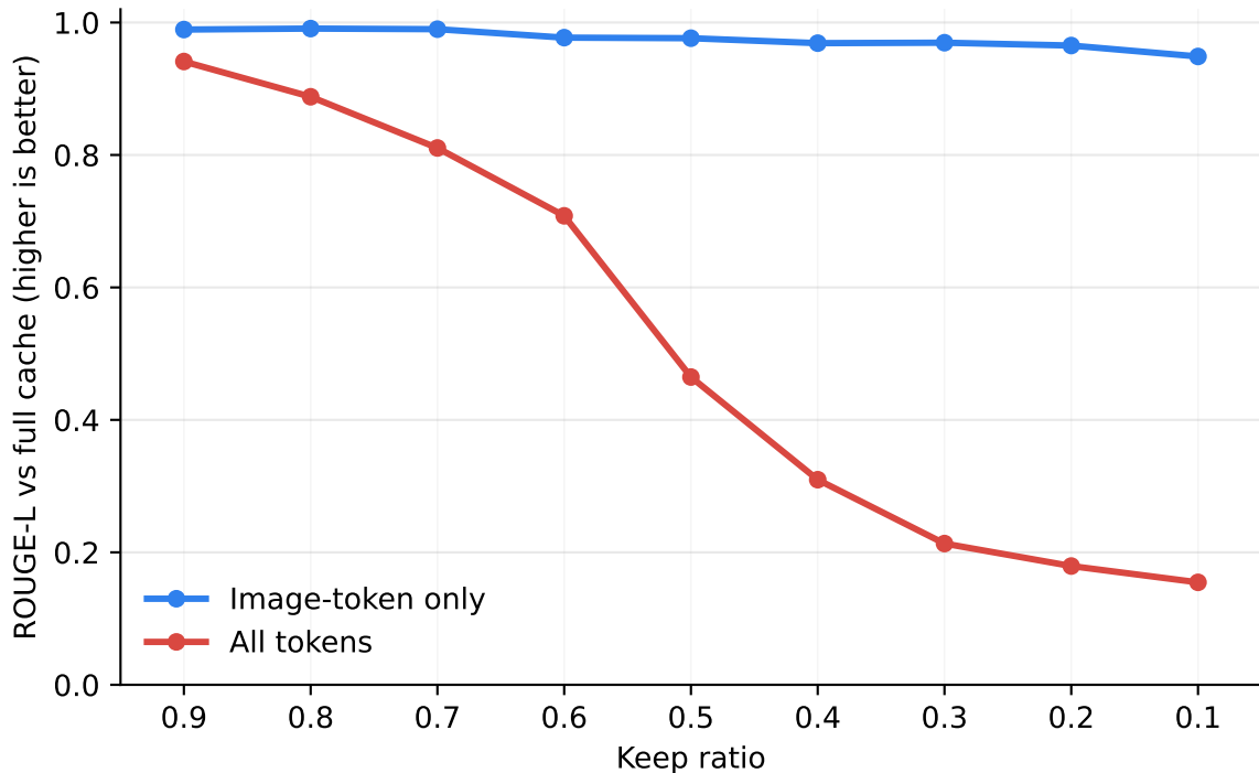
DocVQA random eviction: ROUGE-L
