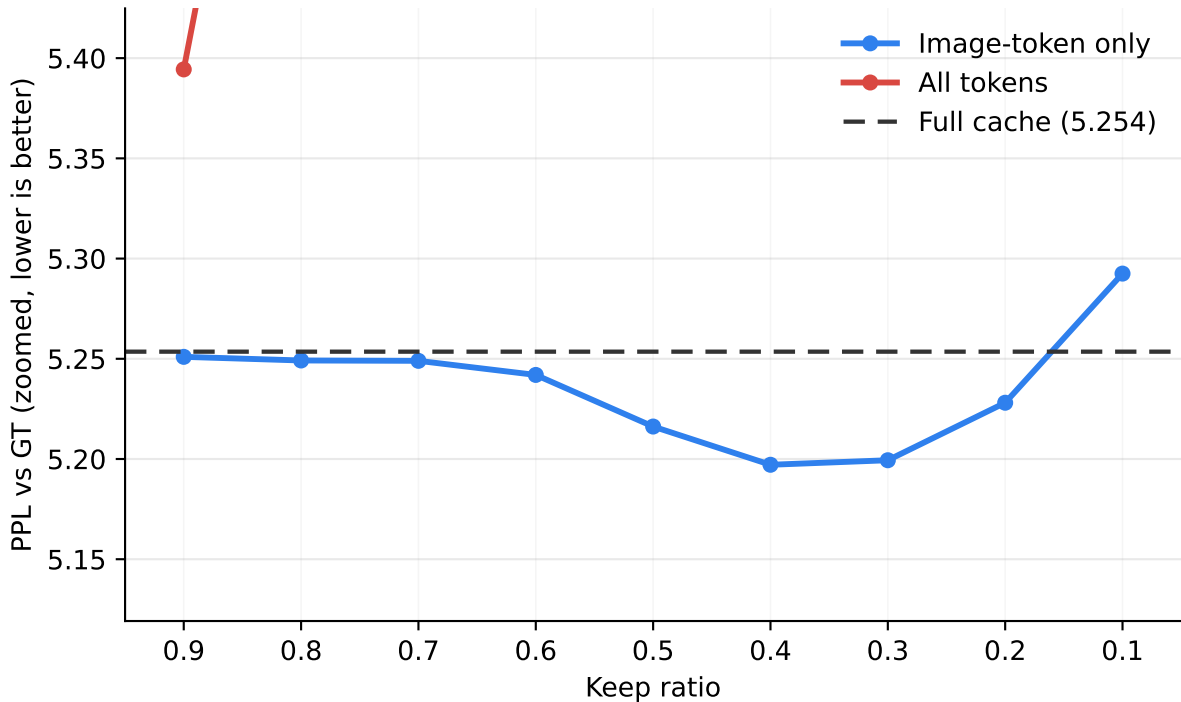
mm-vet random eviction: PPL zoom
