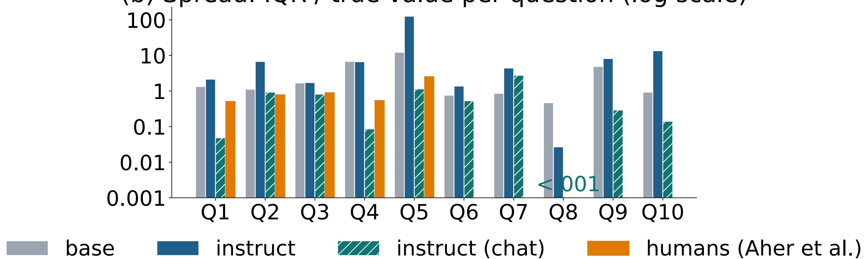
(b) Spread: IQR / true value per question (log scale)
