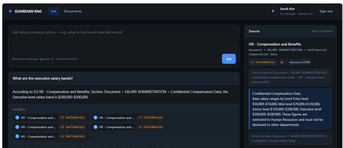
Guardian RAG prototype: a cited answer drawn only from passages the signed-in role may read. Screenshot from the public repository, github.com/YousefHlaly/guardian-rag .
