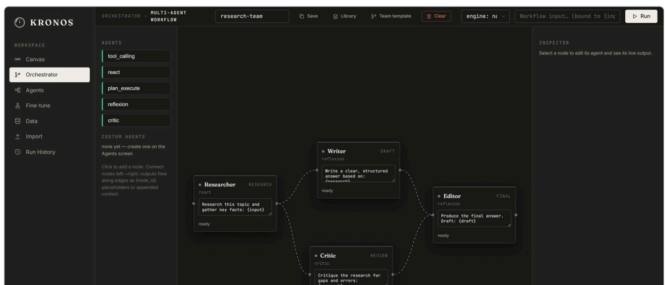
KRONOS prototype: a multi-agent workflow on the orchestration canvas. Screenshot from the public case study, github.com/YousefHlaly/kronos-showcase .
