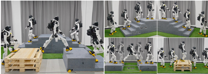
Figure 8: Key frames of zero-shot real-world lab-level deployment. SSR enables stair traversal, crossing a 90 cm gap, and climbing onto a 45 cm platform with safe foot placement and natural whole-body motion.
