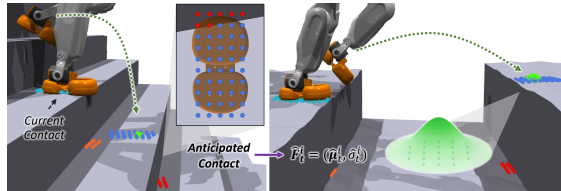
Figure 3: Imagined foothold guidance. We measure support deficiency over a sole-sized terrain patch. During swing, a foothold imagination model estimates anticipated foothold distributions for dense guidance.
