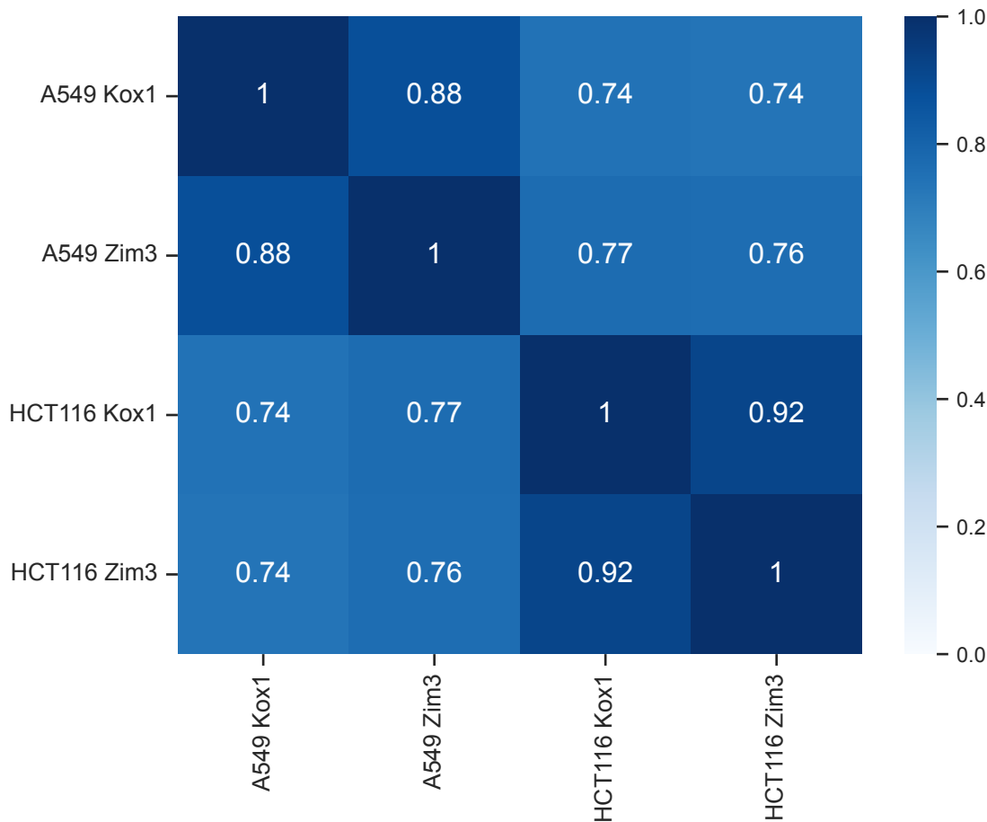
Correlation between guide z-scores
