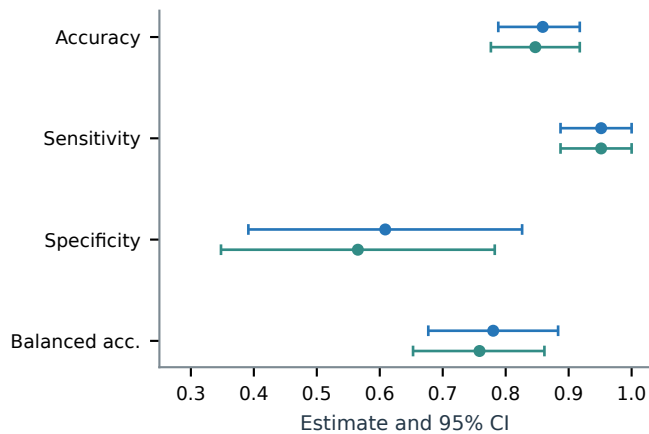
b Threshold-based performance
