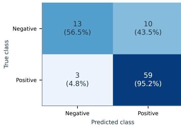
d Equal-weight fusion
