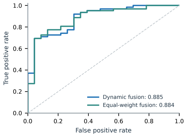
a Patient-level ROC curves
