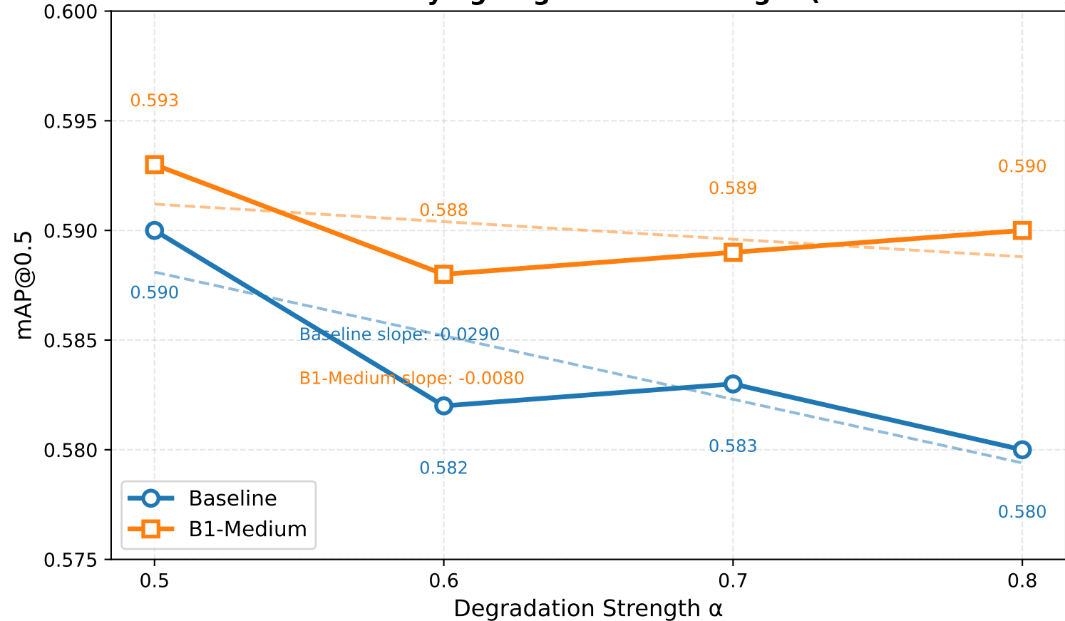
Performance under Varying Degradation Strength (DMZ Dark Subset)
