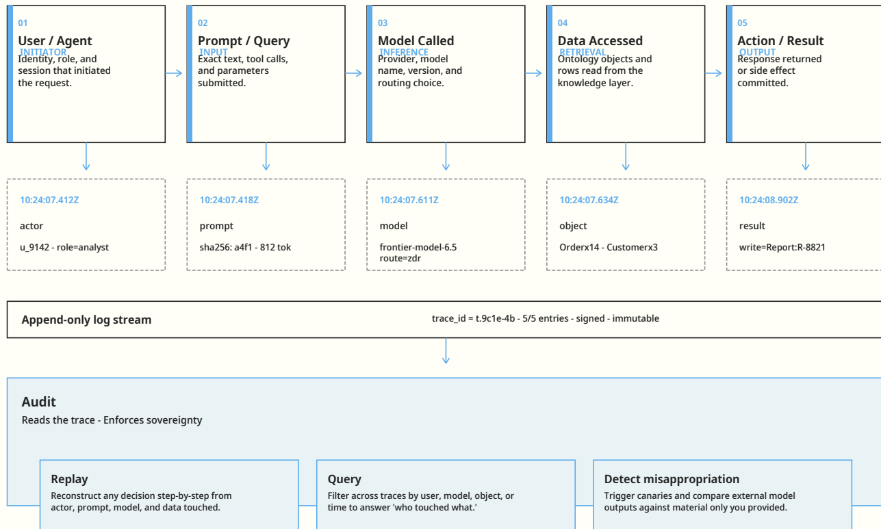
Fig. 12 Audit & Logs
