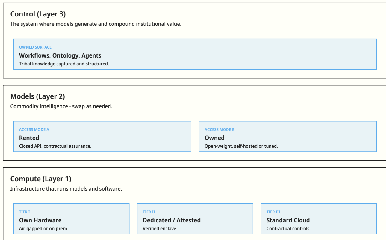
Fig. 3 Architecture Layers
