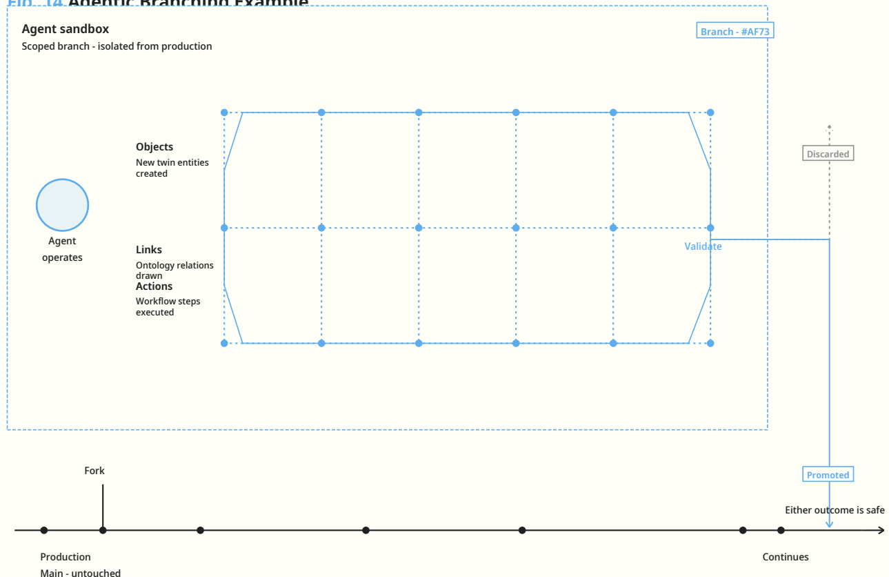
Fig. 14. Agentic Branching Example
