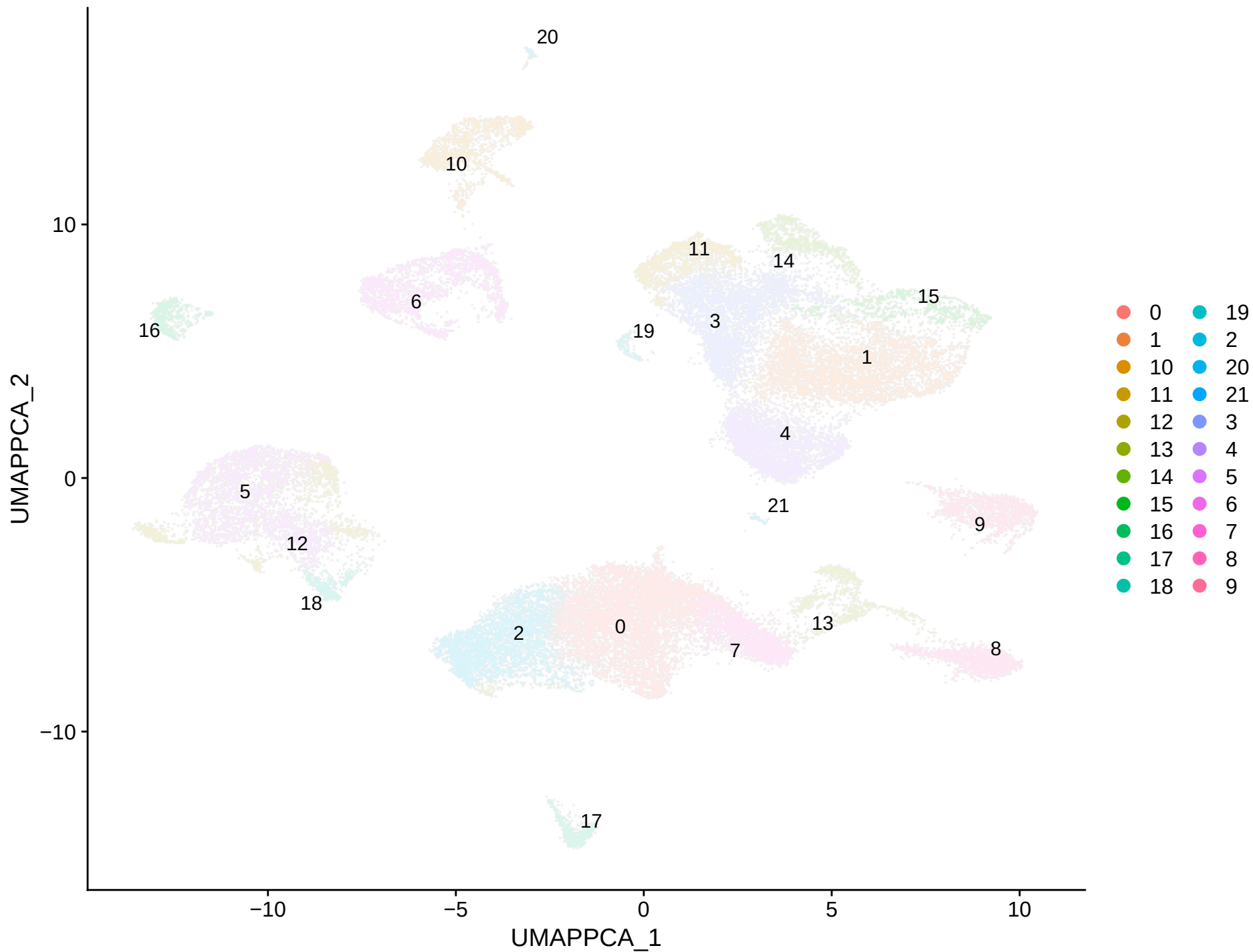
04b PCA-UMAP: clustering resolution = 0.5
