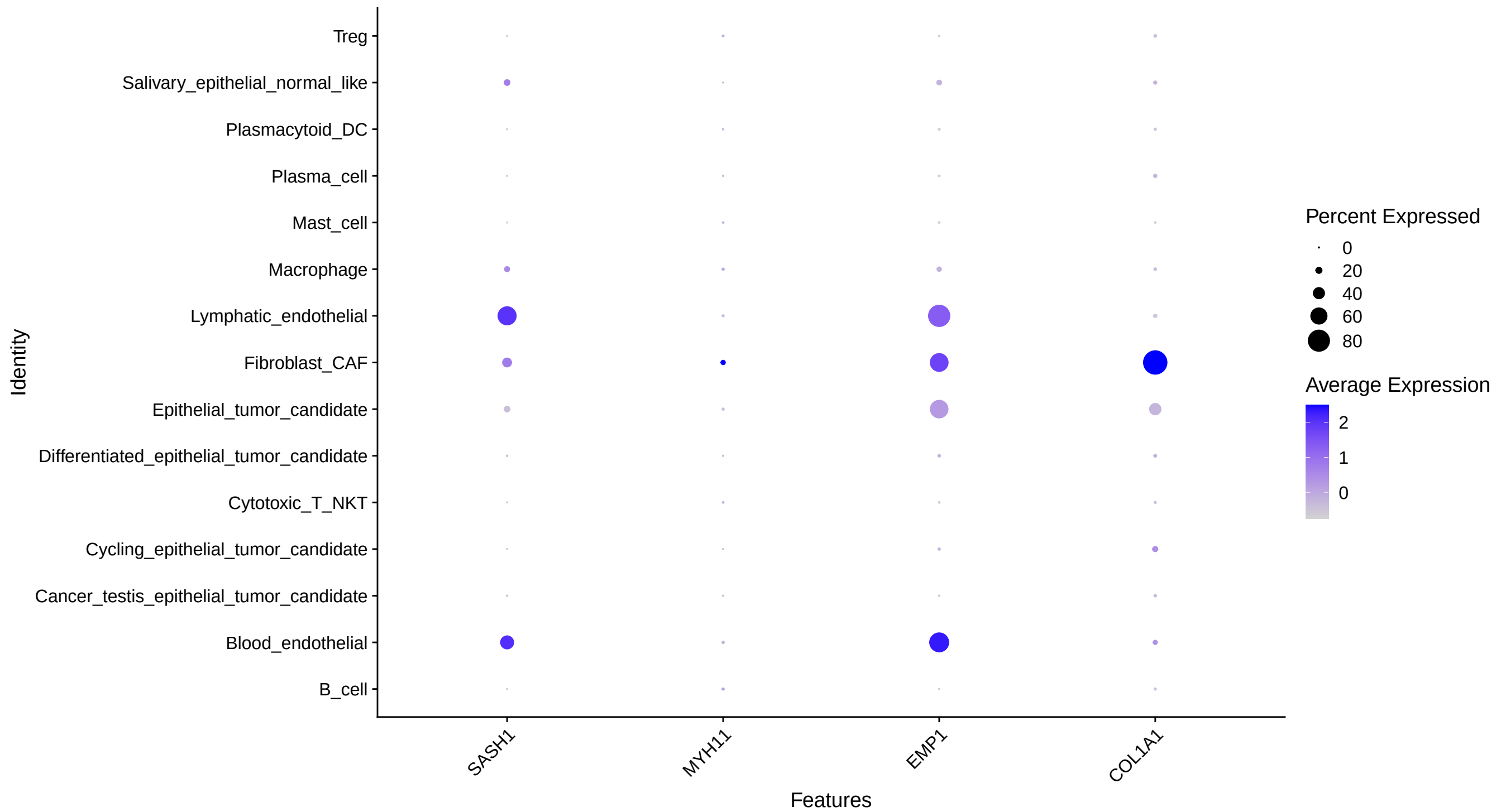
Core genes across manually annotated cell types
