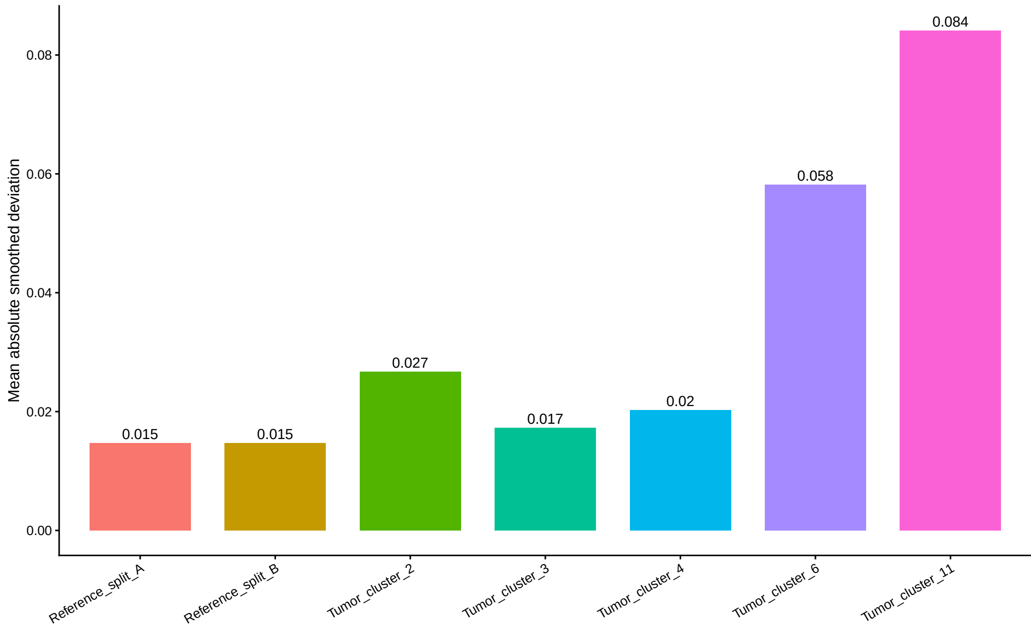
Chromosome-aware expression deviation score
