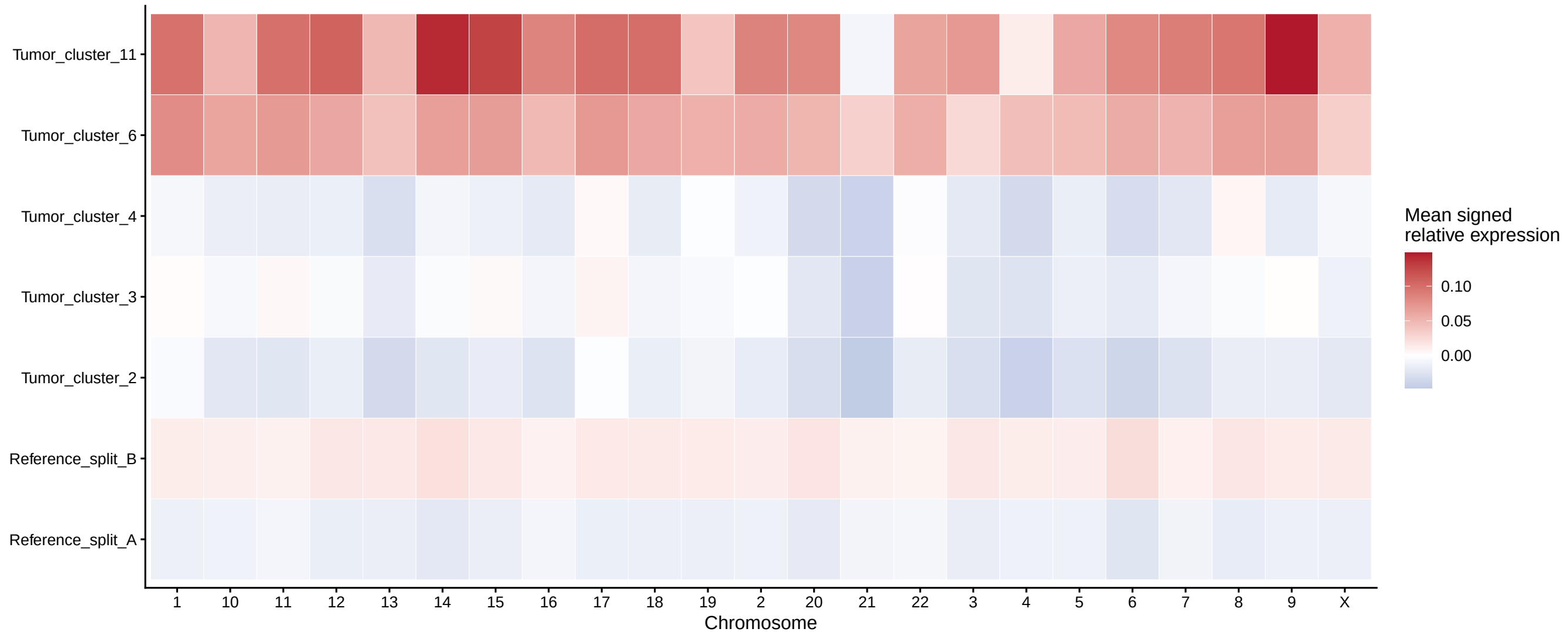
Chromosome-level relative-expression deviation
