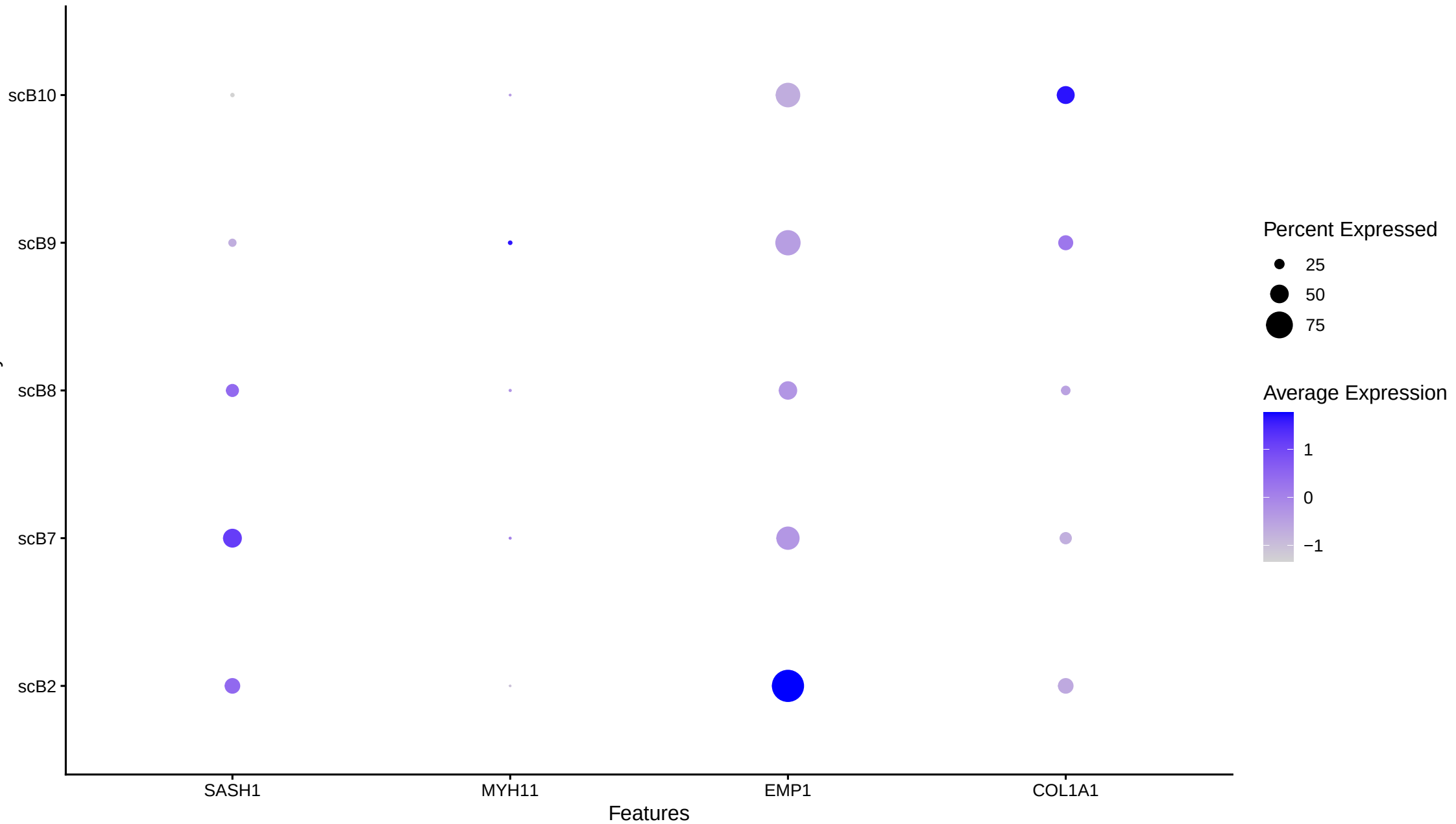
Core genes across samples in cluster6 strict malignant cells
