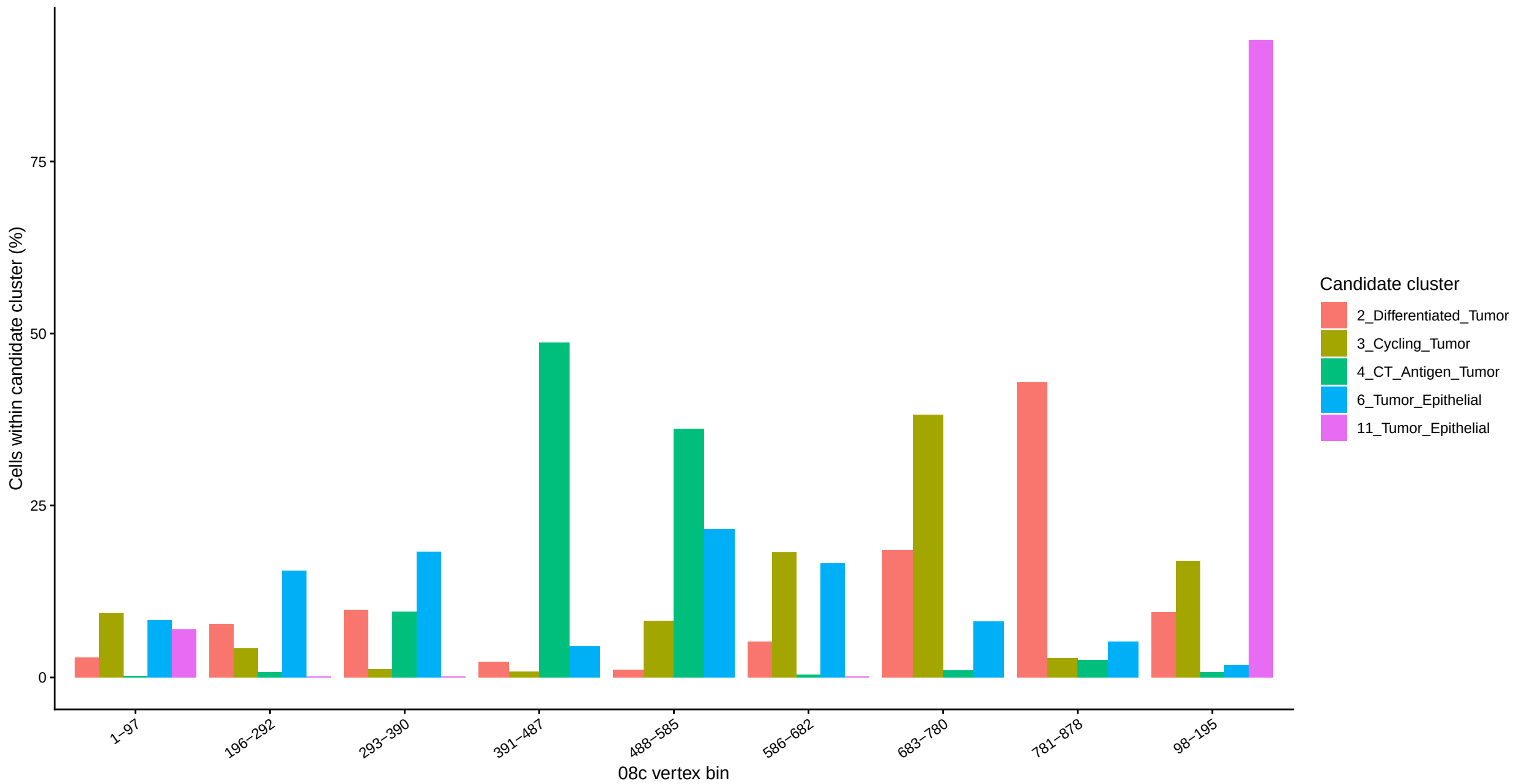
Vertex-bin Distribution of Candidate Tumor-Related Clusters
