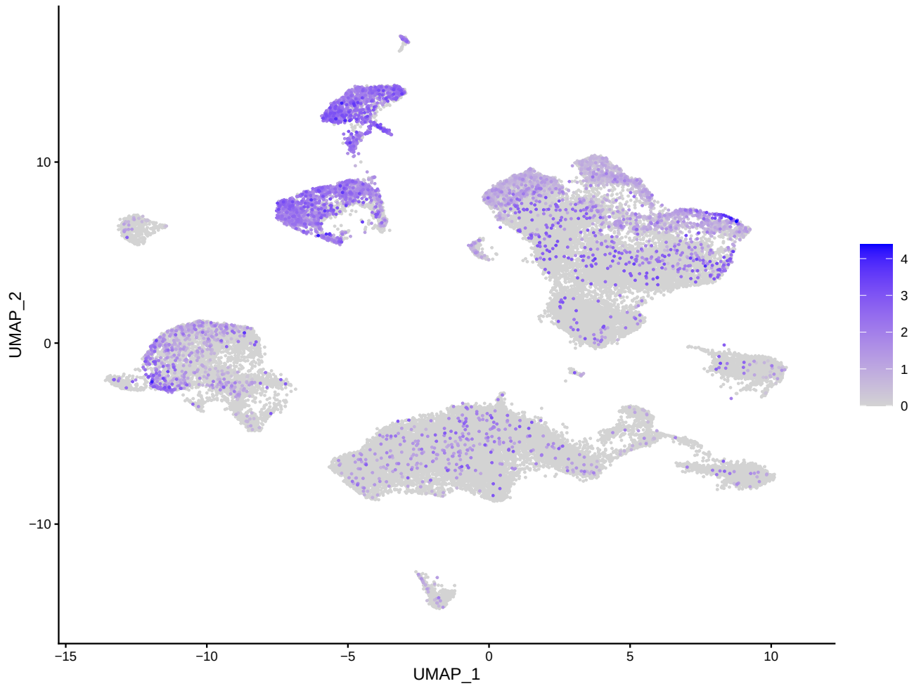
EMP1 FeaturePlot
