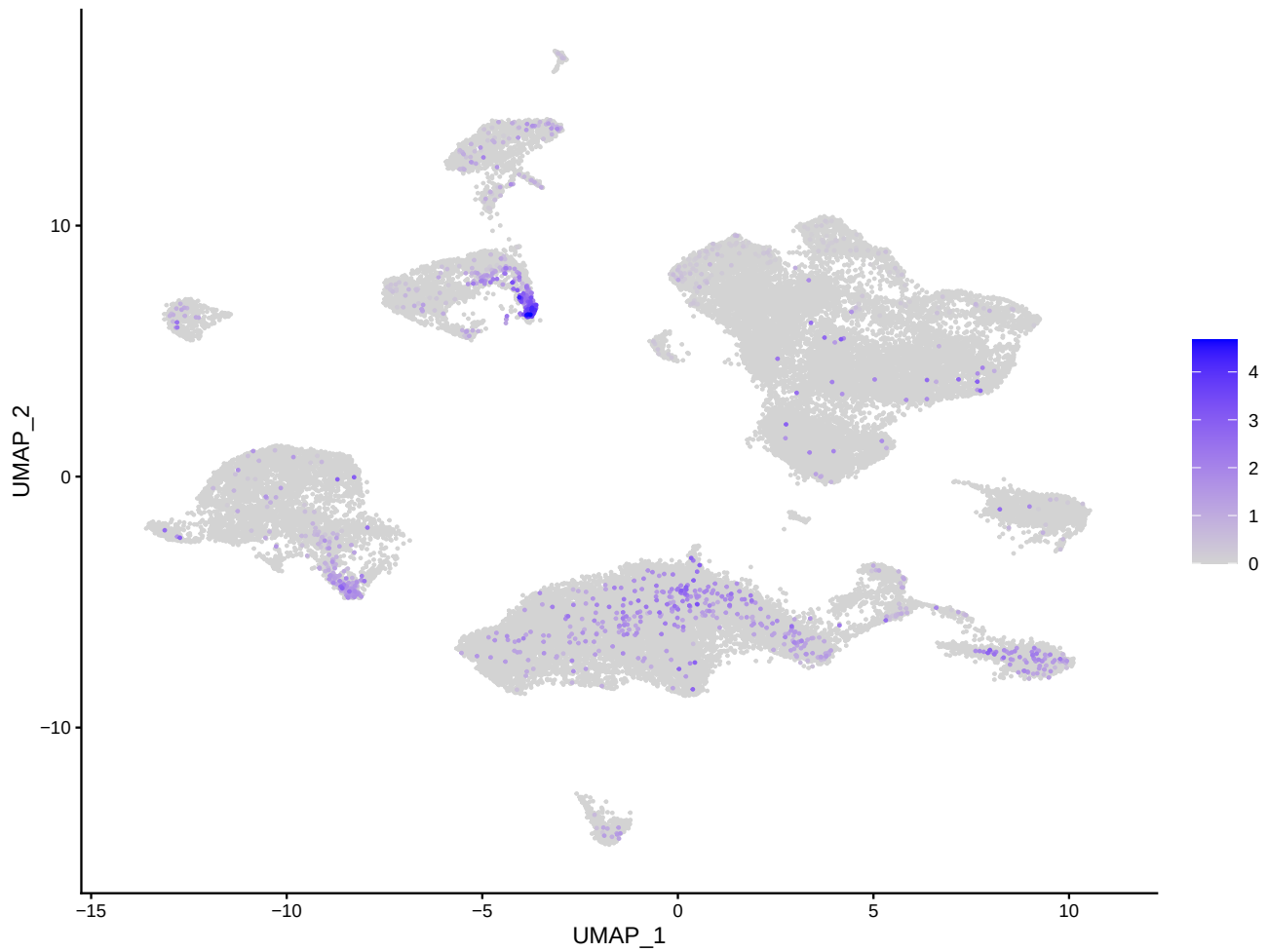
MYH11 FeaturePlot
