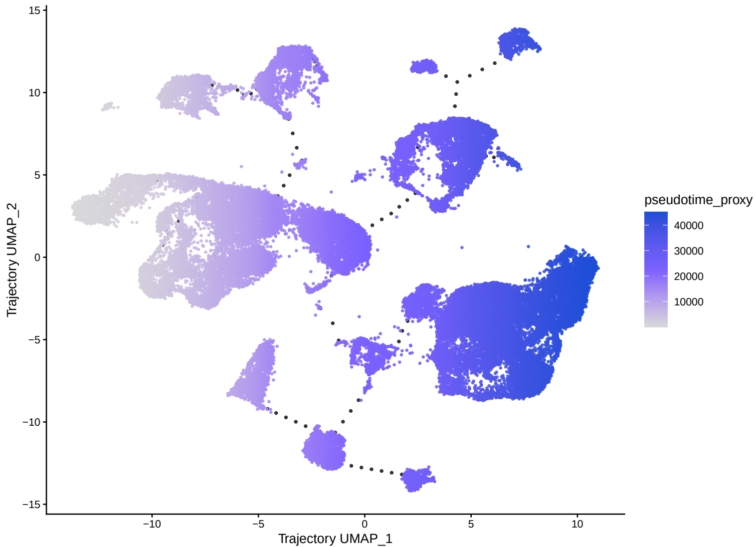
Supplementary pseudotime/proxy
