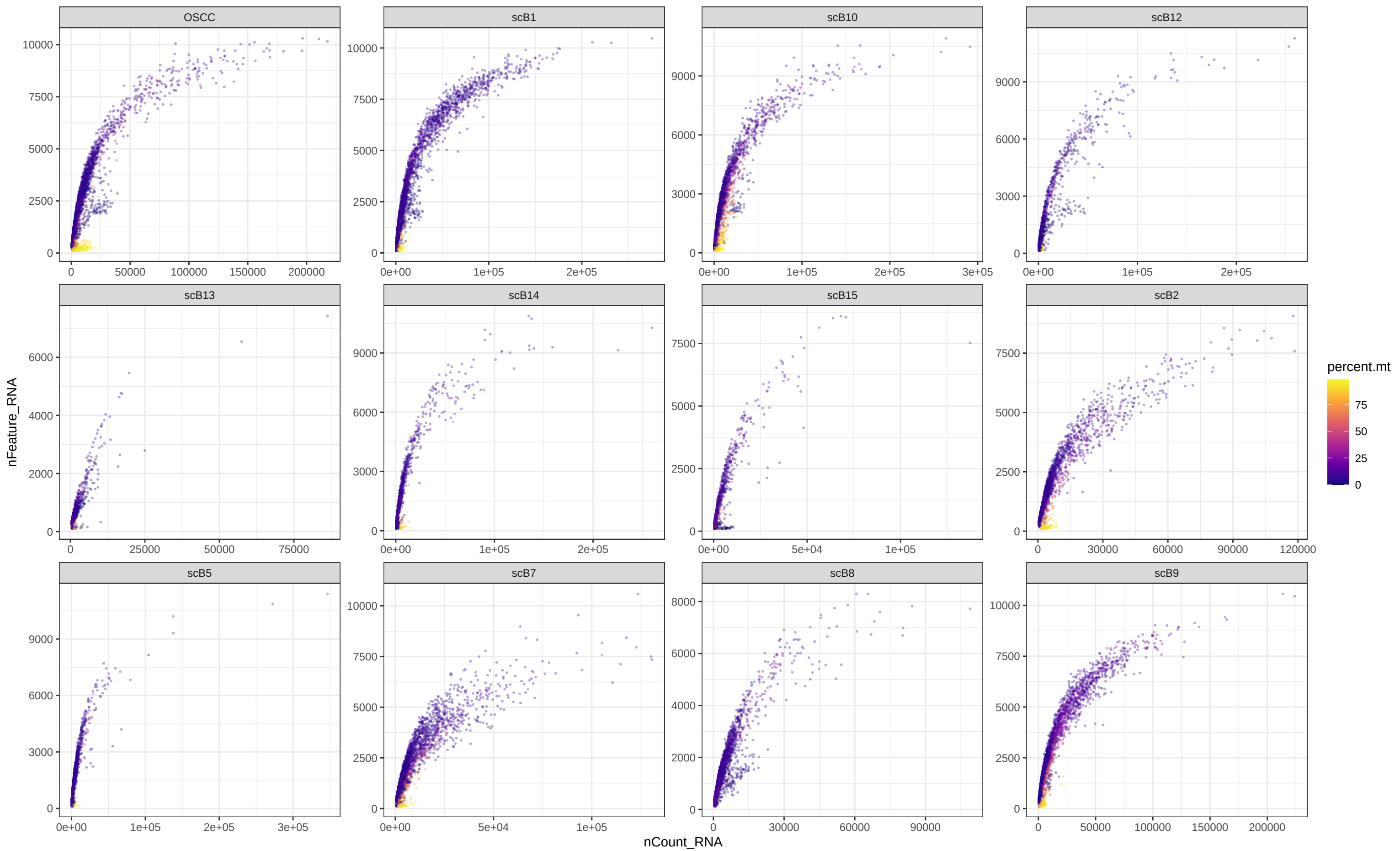
QC: UMI counts versus detected genes
