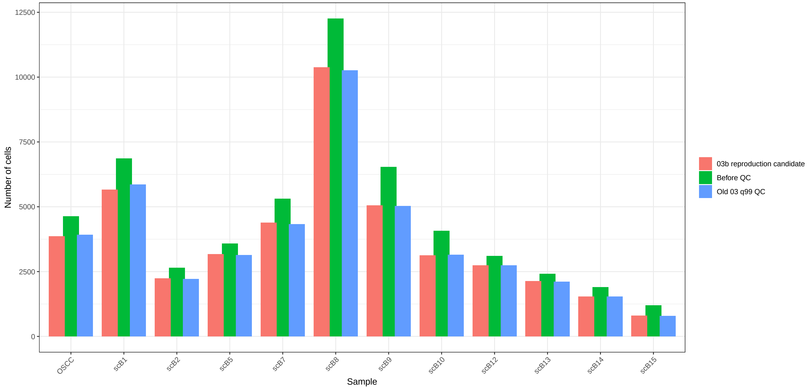
Cell number comparison: old 03 versus 03b QC
