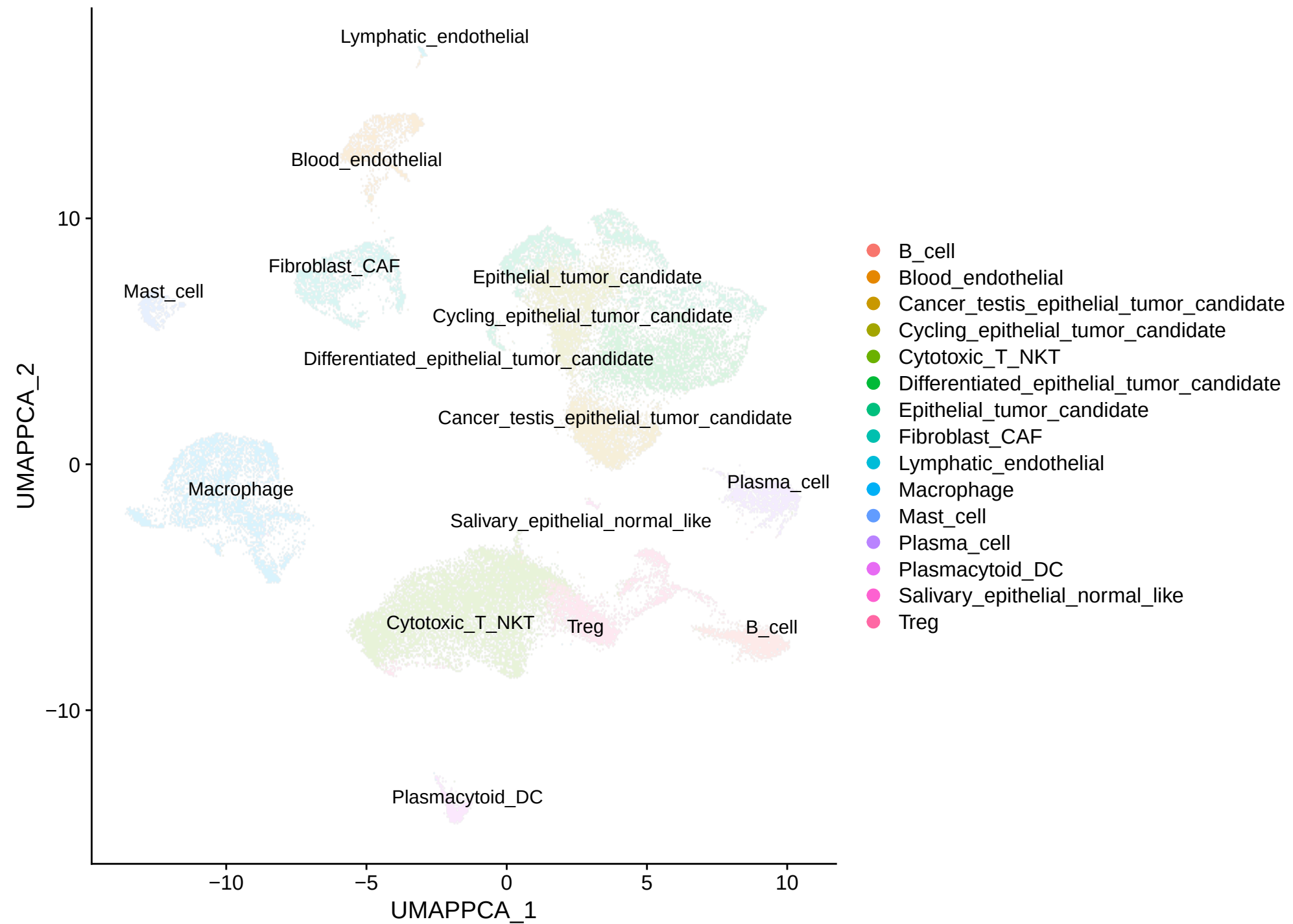
PCA-UMAP by manual cell-type annotation
