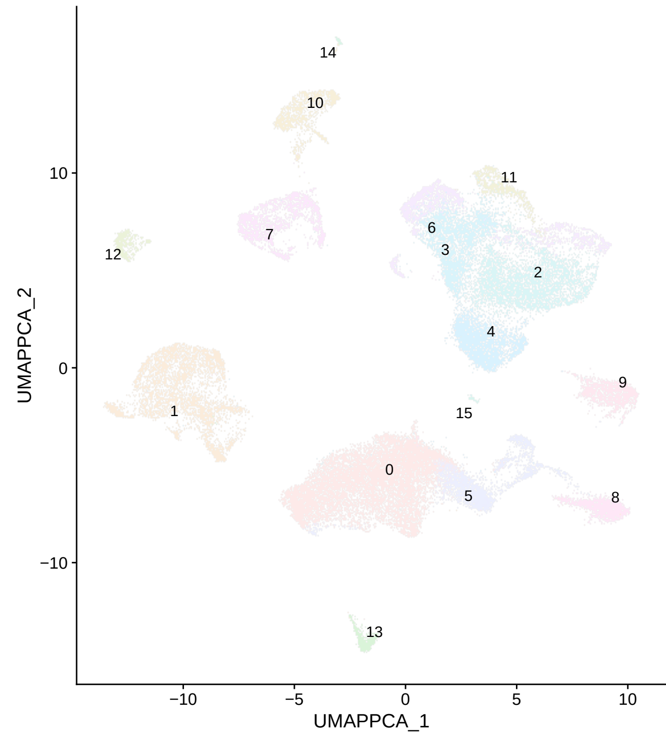
PCA-UMAP by cluster
